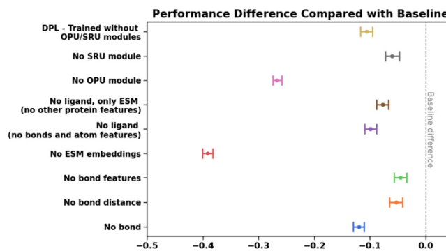
FIG. 8. Ablation studies on ProteinReDiff's model architecture and featurization. The dash line indicates the baseline's average score obtained from ProteinReDiff without ablations.
