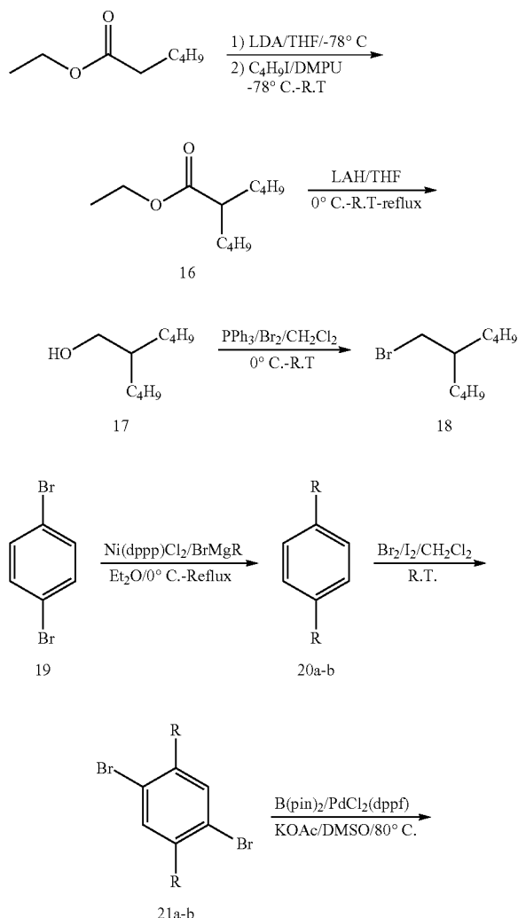
Scheme 4. Synthetic route for compounds 20a-b and 26.
