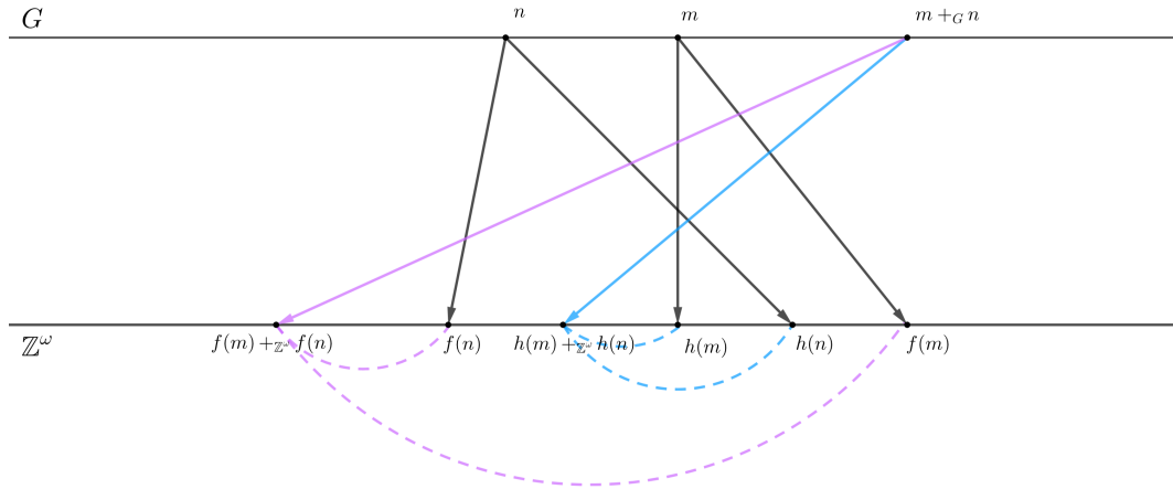
Figure 3.1: A visual representation of Lemma 3.1
