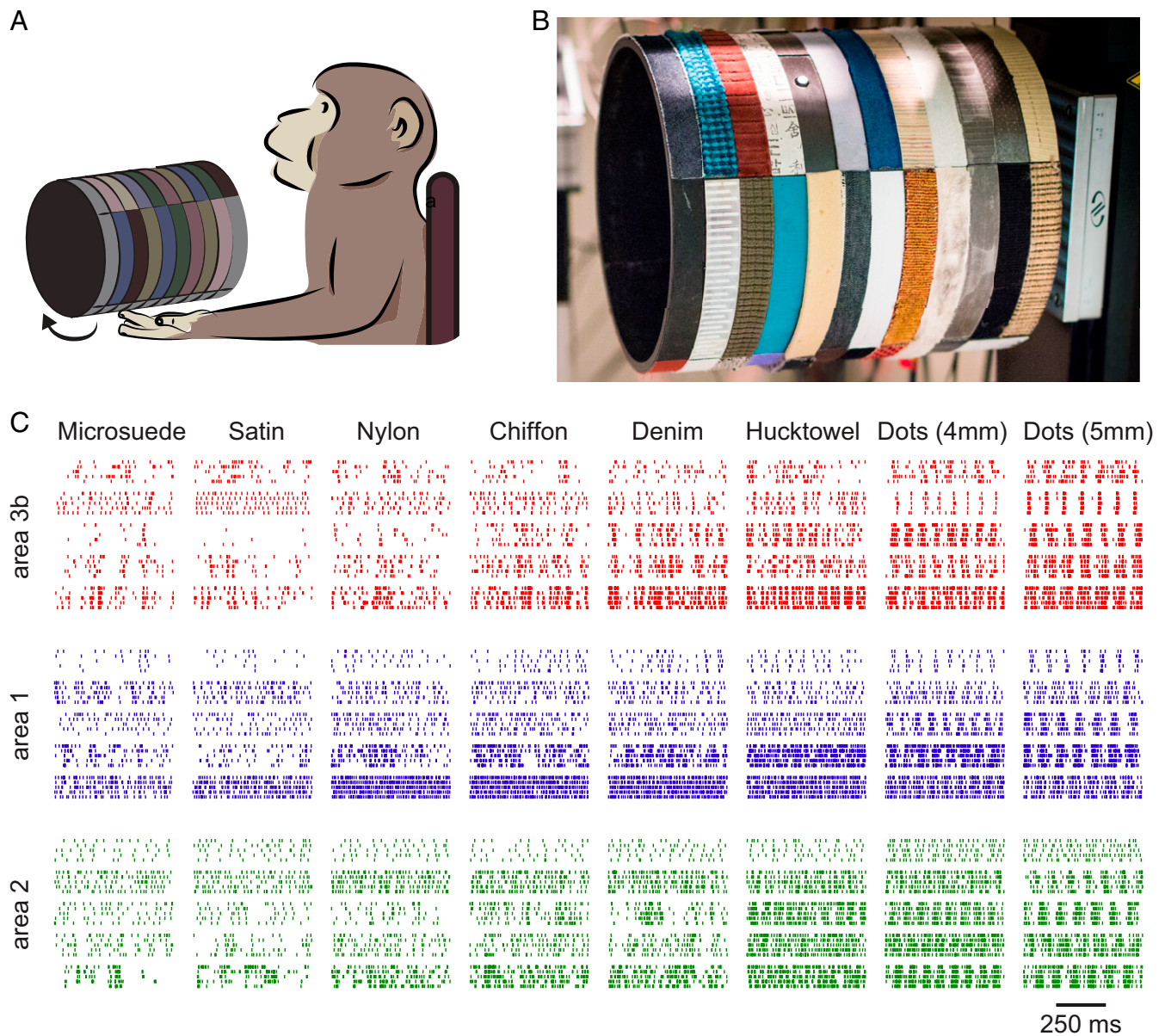
Fig. 1. Experimental apparatus and sample texture responses. (A) Textures were passively presented to the distal finger pads of awake macaques. (B) The rotating drum stimulator—on which the 59 textures were mounted—allows a surface to be scanned across the fingertip at a precise and repeatable speed and depth of indentation into the skin. (C) Sample spiking responses of five neurons each in areas 3b, 1, and 2 to five repetitions of eight textured surfaces.
