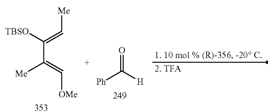
Scheme 4 - Enantioselective HDA Reactions of Aldehydes with a Metal Catalyst
