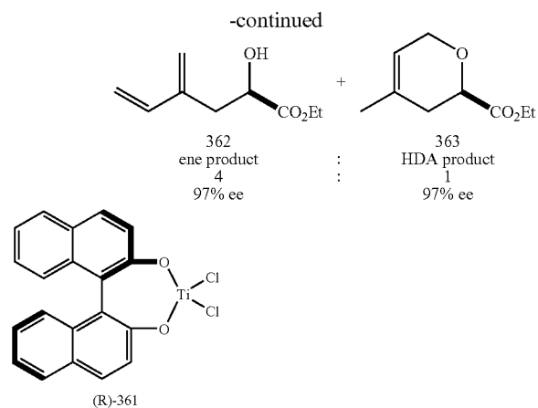
Scheme 7 - Chemoselective HDA Reactions Catalyzed by Metal Catalyst
