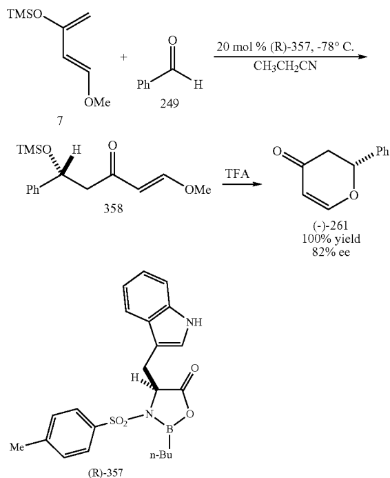
Scheme 5 - HDA Reactions Catalyzed by Tryptophan-derived Lewis Acid Catalyst
