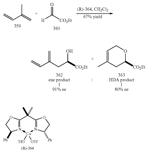
Scheme 7 - Chemoselective HDA Reactions Catalyzed by Metal Catalyst
