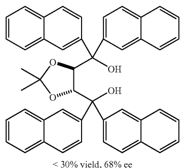
Scheme 10 - Results with Naphthyl-TADDOLs
