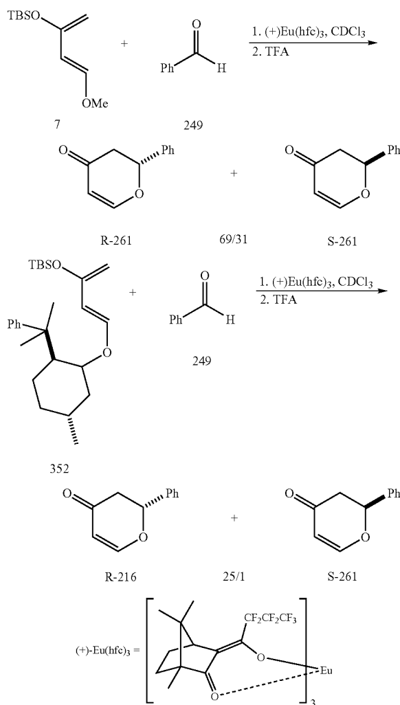
Scheme 3-Enantioselective HDA Reactions Catalyzed by a Metal Catalyst.
