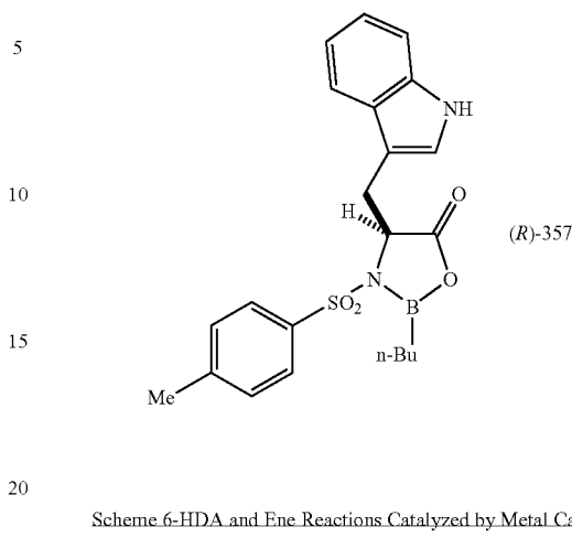
Scheme 4- Enantioselective HDA Reactions of Aldehydes with a Metal Catalyst
