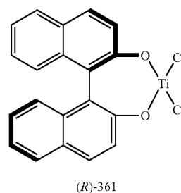
Scheme 7- Chemoselective HDA Reactions Catalyzed by Metal Catalyst
