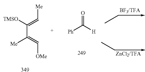
Scheme 2-Asymmetric Diels-Alder reactions with a Lewis Acid catalyst.
