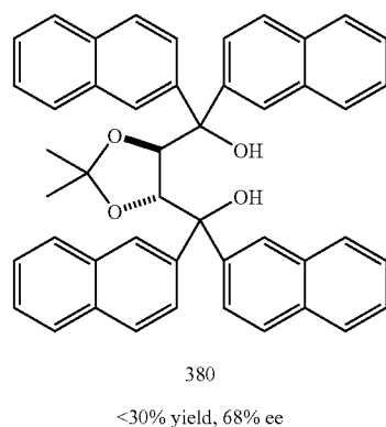
Scheme 10-Results with Naphthyl-TADDOLs
