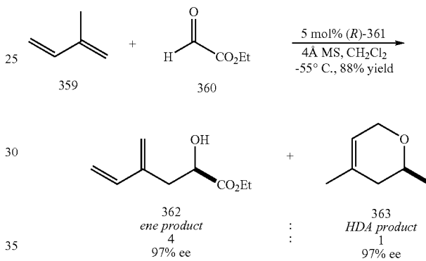
Scheme 6- HDA and Ene Reactions Catalyzed by Metal Catalysts
