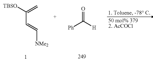
Scheme 9-Initial Result with TADDOL 379
