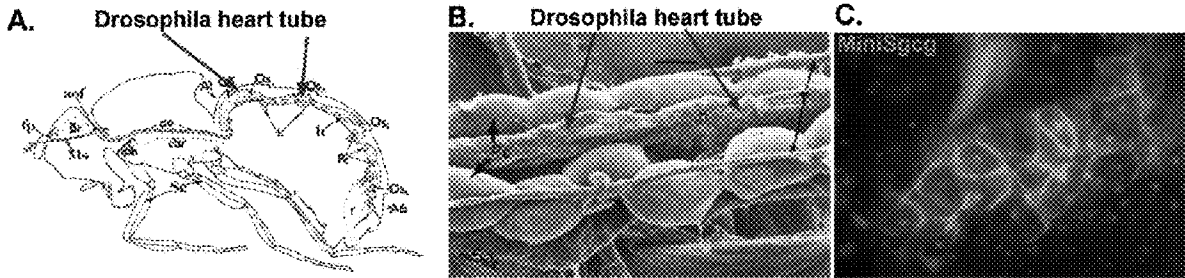
A and B from Curtis NJ J. Morphology 1999 240:225
