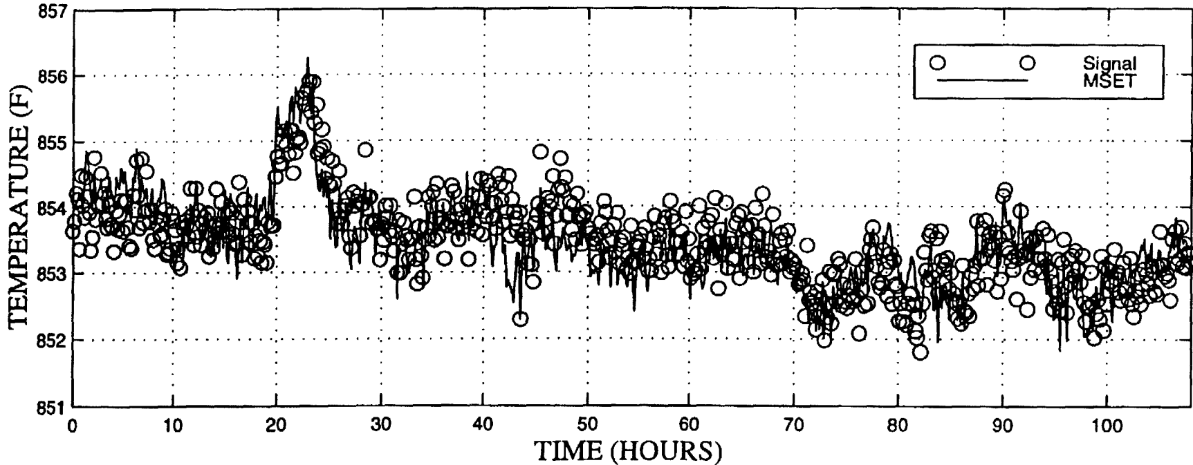
(CHANNEL(7)) SUBASSEMBLY OUTLET TEMPERATURE 1A1
