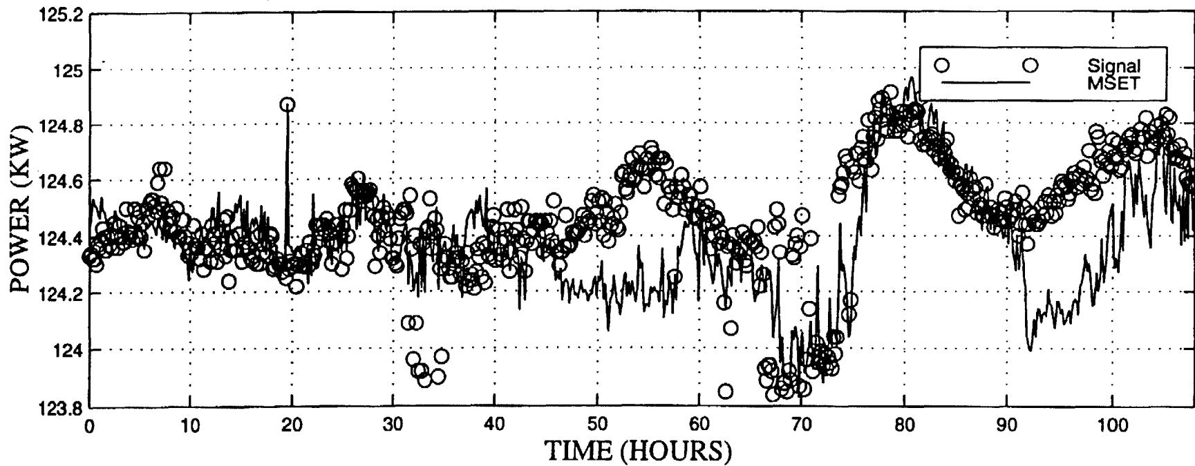
(CHANNEL(2)) PRIMARY PUMP #2 POWER
