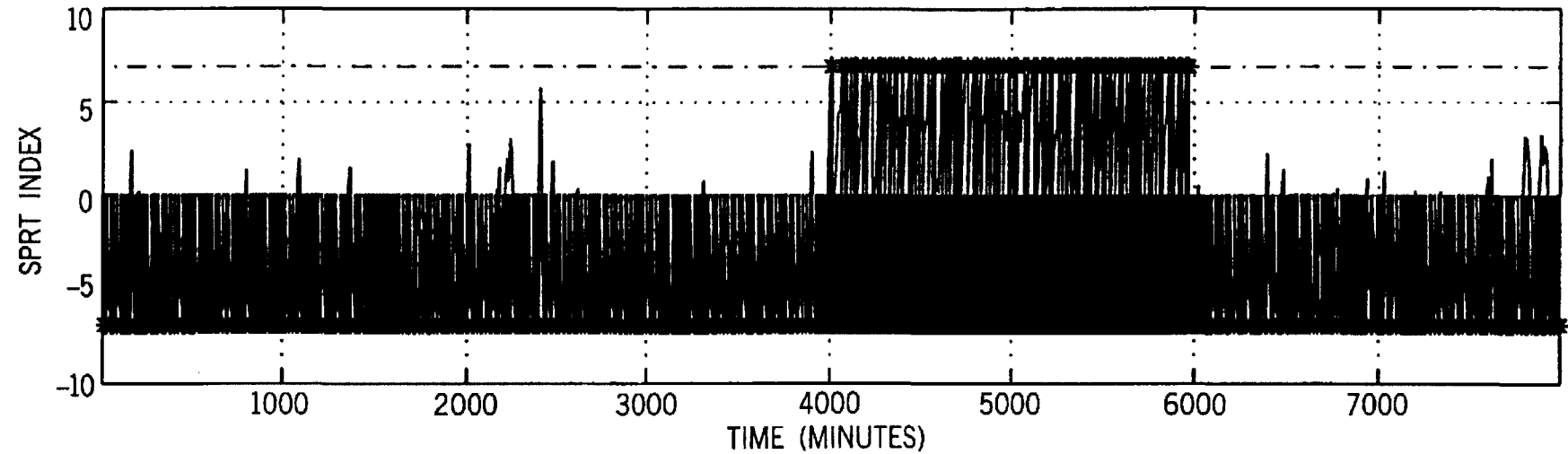
(#3) EBR-II, SUBASSEMBLY OUTLET TEMPERATURE (5C2) SPRT RESULTS
