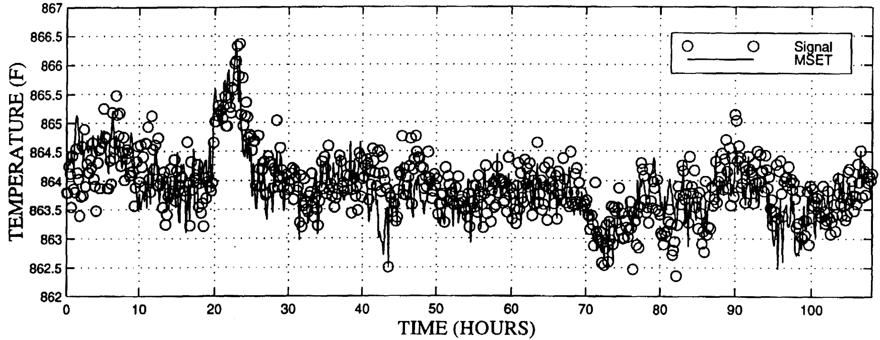
(CHANNEL(11)) REACTOR OUTLET TEMPERATURE 1534CF
