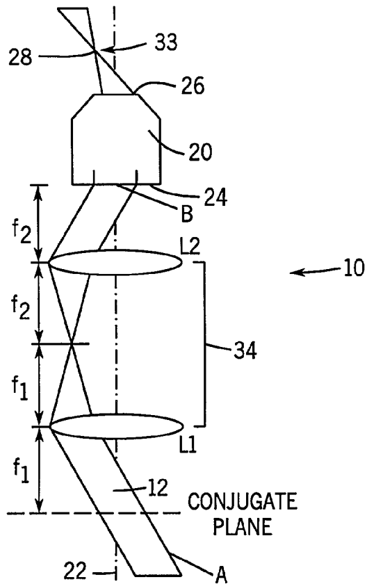
FIG. 2 PRIOR ART
