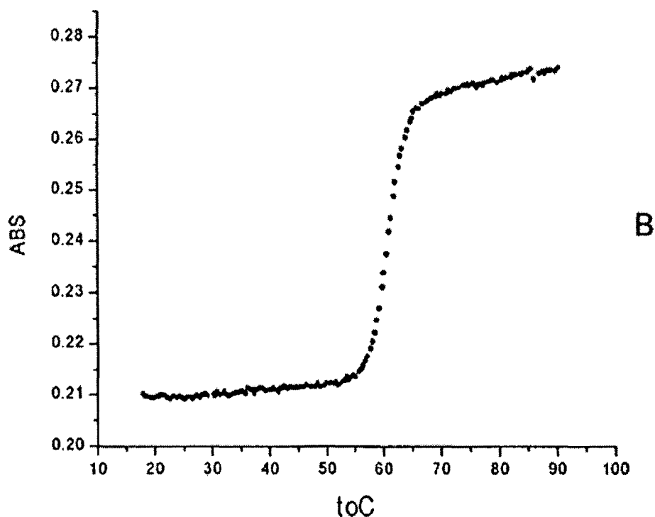
B. Melting curve of the Duplex 4 (Scheme 3, Fig.6 cont) ABS- absorbtion, t °C – temperature in Celsius
