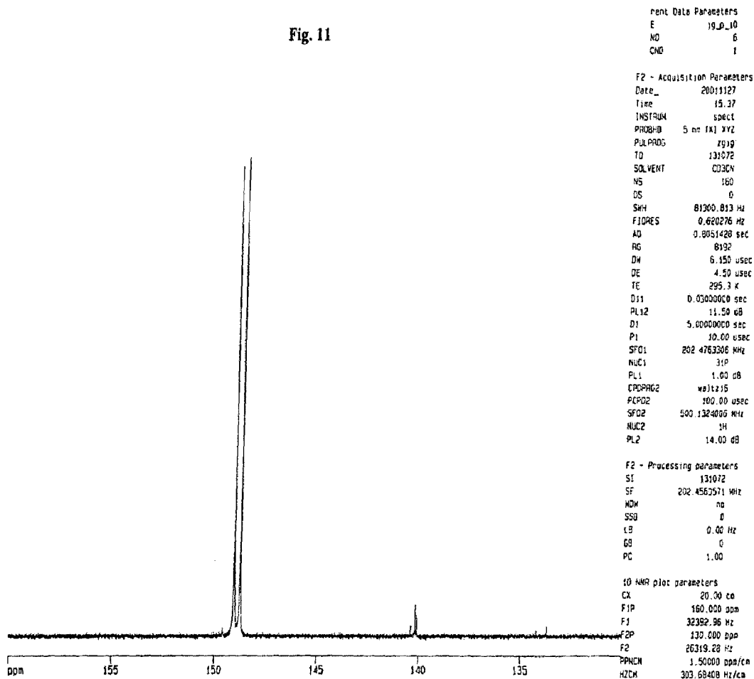
31 P NMR Spectrum of Connector Phosphoramidite (7)
