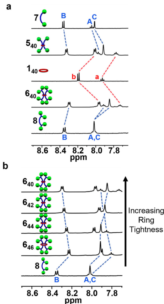
Fig. 7 Partial 1 H-NMR overlay (500 MHz, CDCl 3 , 25 °C) of (a) [3]rotaxanes 5 40 and 6 40 and their free components 1 40 , 7, and 8 and (b) [3]rotaxanes 6 40-46 and dumbbell component 8 (labels correspond to Fig. 1).
