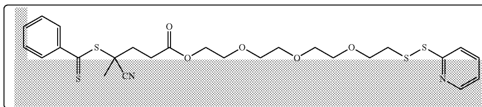
Compound (RAFT Agent) 20
