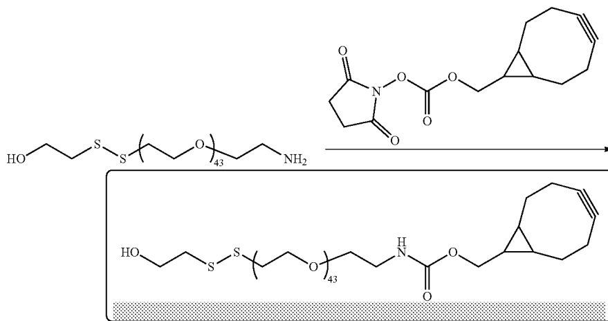
BCN PEG 43 disulfaneyl ethanol
