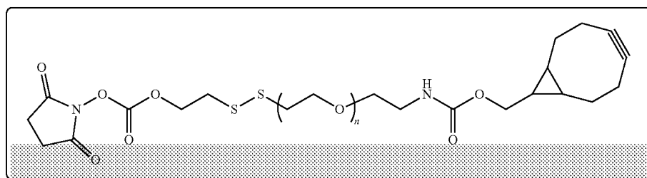
BCN—PEG2K—NHS
