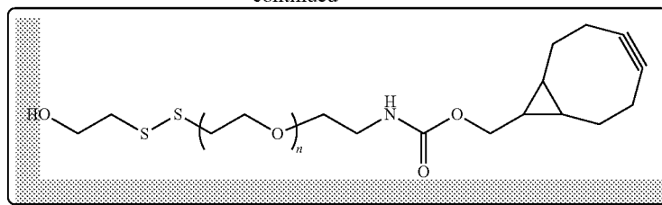
PEG2K—BCN disulfaneyl ethanol
