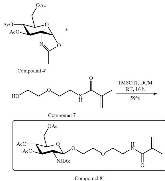
(2-(2-hydroxyethoxy)ethyl)methacryloyl 2-acetamido-3,4,6-O-acetyl D-glucoside (8')
