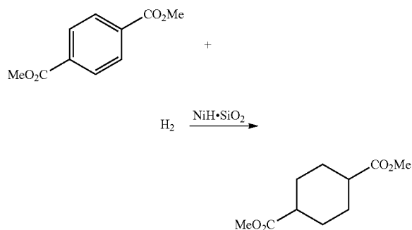
Hydrogenation of Dimethyl Terephthalate using Metalated Silica Catalyst.
