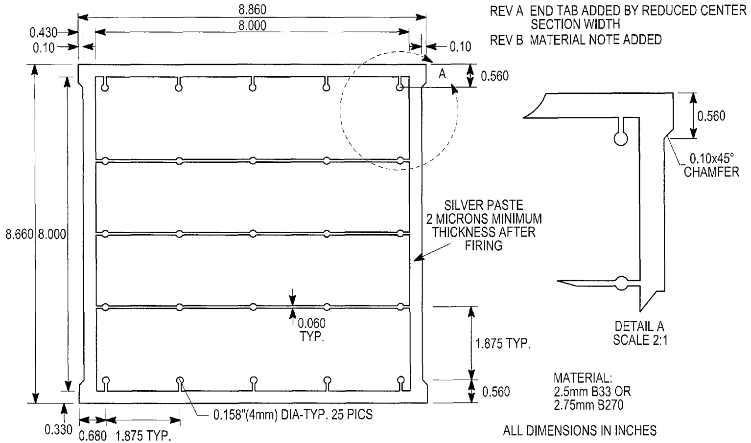
WINDOW HIGH VOLTAGE DISTRIBUTION PATTERN
