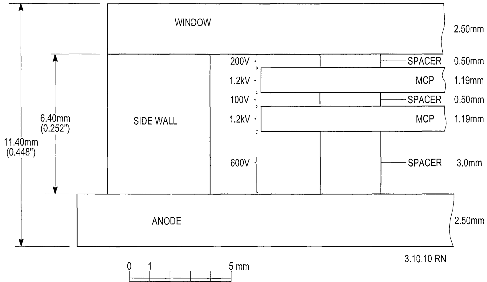
BASE LINE MCP-PMT STACKUP
