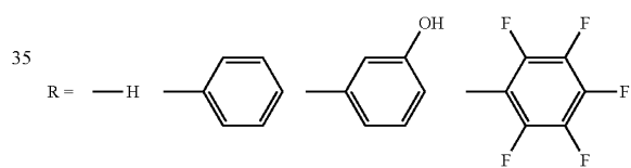
DBP, DBC, DBBC ligands and their derivatives
