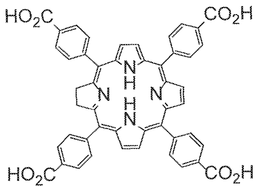
5,10,15,20-tetra(3',5'-dicarboxylphenyl)porphyrin
