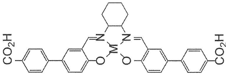
disalicylidene-1,2-cyclohexyldenediamine complex
