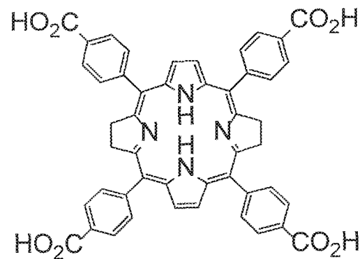
5,10,15,20-tetra(p-carboxylphenyl)bacteriochlorin
