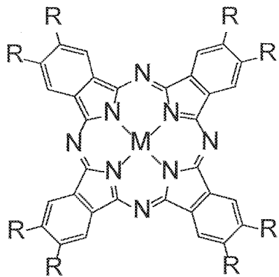
5,10,15,20-tetra(p-pyridyl)porphyrin
