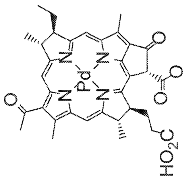
Padoporfin (Tookad)
