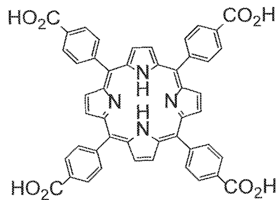
5,10,15,20-tetra(p-carboxylphenyl)porphyrin
