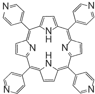
5,10,15,20-tetra(p-pyridyl)porphyrin
