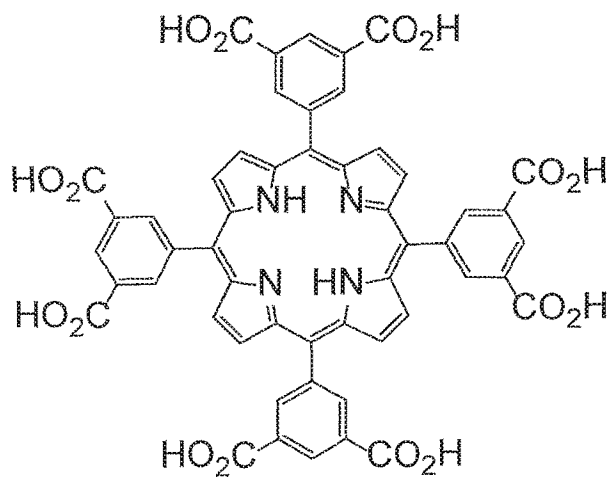
5,10,15,20-tetra(3',5'-dicarboxylphenyl)porphyrin
