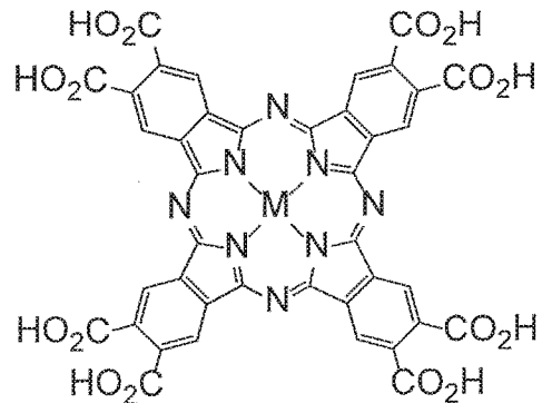
Phthalocyanine-octacarboxylic acid
