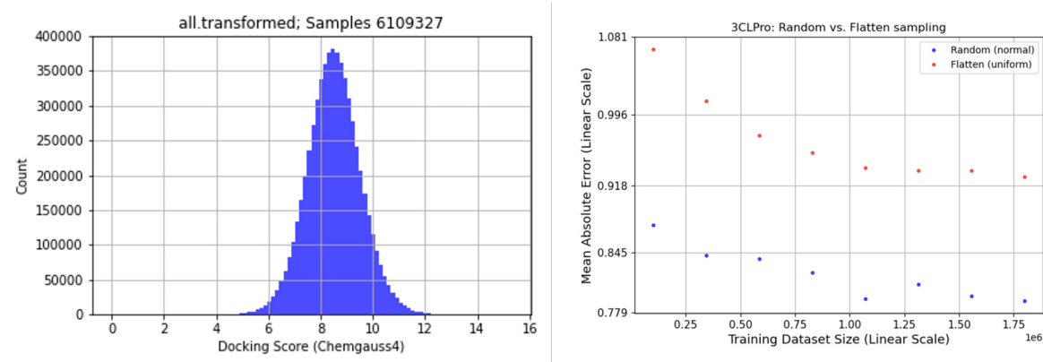
Figure 5.1: (left) Histogram of protein-ligand docking of transformed docking scores for 3CL-M pro . The distribution is from the ORZ dataset based on the transformed 2D scores. (right) Learning curve between dataset size and MAE between random and flattened datasets .
