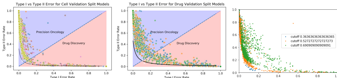
Figure 3.4: Error trade-off. type I error (false positive rate) vs type II error (false negative rate) tradeoff for cell validated models (left) and drug validated models. Cut-off analysis is presented (right) for drug validated models, where the boundary of the error trade-off curve can be shifted with post-processing for even finer control over virtual screening error.
