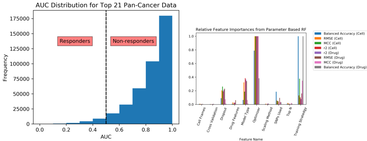
Figure 3.3: Distributions of labels and feature importance. (Left) The AUC distribution of pan-cancer data frame. With this scheme, the training distribution has 3.86% responders. While our cutoff of 0.5 is arbitrary, learning to distinguish this slice along with a regression-based training strategy will prevent standard regression metrics from appearing much better than they are on the skewed portion of the dataset. (Right) Relative feature importance for hyperparameters used in model training for predicting validation metric using decision trees. The r^2 for those models were > 0.9 on cell validation metrics, and > 0.6 for drug validation metrics. Optimizer, model type, and dropout were among the top three features, though the training strategy very important when predicting balanced accuracy.
