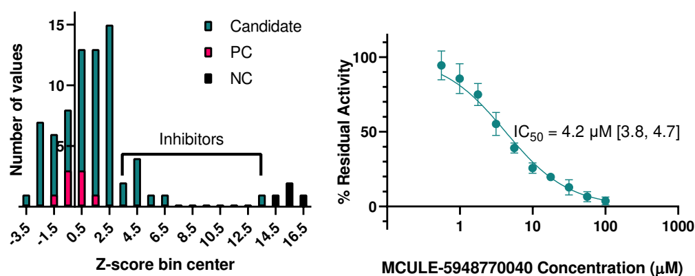
Figure 4.5: Plate-based \text{M}^{\text{Pro}} activity inhibition screening and hit confirmation. (A) Histogram of z-scores of candidate inhibitors, no enzyme negative controls (NC), and no inhibitor positive controls (PC). (B) Inhibition of \text{M}^{\text{Pro}} activity in vitro with increasing concentration of MCULE-5948770040. Initial rates are normalized to no inhibitor control (100% activity) and no enzyme control (0% activity). Error bars are standard deviation of two independent experiments, each performed in triplicate. Lines indicate the nonlinear regression of the [Inhibitor] vs. normalized response \text{IC}_{50} equation to the data with GraphPad Prism. Bracketed values indicate 95% confidence intervals from the regression.
