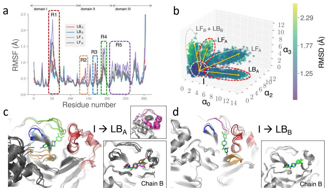
Figure 4.7: Conformational changes upon MCULE-5948770040 binding to M^{\text{pro}} indicate changes within distinct regions, both close-to and farther-away from the primary binding site. (a) RMS fluctuations of the LF- and LB-state of M^{\text{pro}} show several regions with decreased fluctuations that are highlighted within rounded rectangles. Although several regions within these regions are largely similar, amino-acid residues interacting with the ligand stabilize the binding site. (b) To further quantify the nature of these fluctuations, we characterized the collective motions which shows distinct conformational states sampled by the ligand-free (LF) and ligand-bound (LB) states. The yellow arrows indicate conformational transitions from the average structure towards the distinct conformational states (I, LF A , LF B , LB A and LB B ). These transitions are mapped in (c) I \rightarrow LB A and (d) I \rightarrow LB B . (We show the I \rightarrow LF A and I \rightarrow LF B ). In each case, we observed that M^{\text{pro}} chain B of the dimer was more stable the chain A (insets). Regions highlighted in (a) show the motions undergone by the different regions of M^{\text{pro}} .
