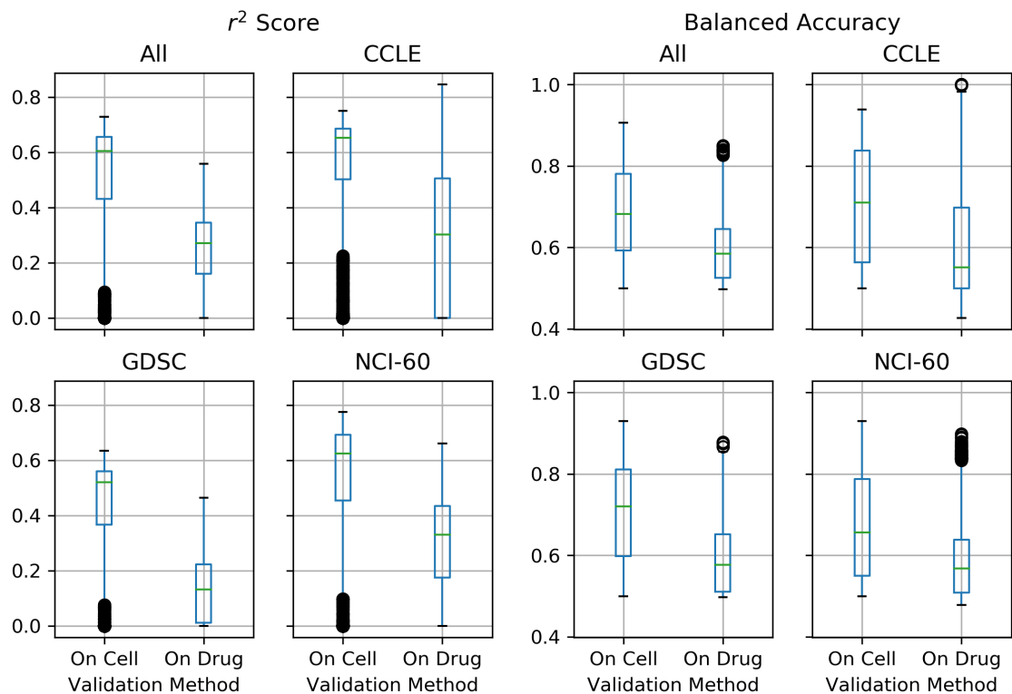
Figure 3.5: Comparison of the models’ performances between validation methods over all converged trained models broken down by sample’s originating study.
