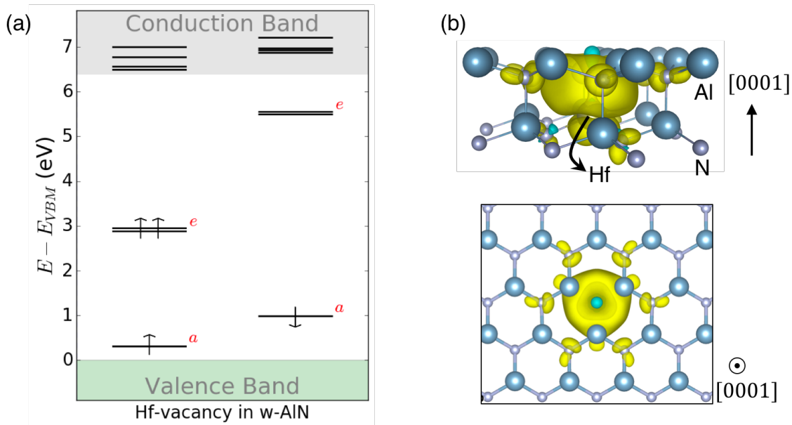
Figure 6.2: Hf-vacancy complex in w-AlN. (a) The defect level diagram of an axial Hf-vacancy in w-AlN calculated at the DDH level of theory. The symmetry of the state is ^3A_2 . In this study, we only consider the axial defect configuration in C_{3v} symmetry. In principle, however, a basal configuration in C_{1h} symmetry is also possible. (b) Side (top) and top (bottom) views of the ground-state spin density of the Hf-vacancy in w-AlN calculated at the DDH level of theory.
