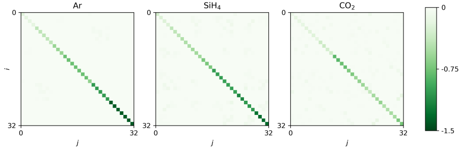
Figure 3.11: First 32 \times 32 matrix elements of the exchange-correlation kernel in PDEP basis (the space of \tilde{\chi}_0 eigenvectors) for Ar, \text{SiH}_4 and \text{CO}_2 molecule.
