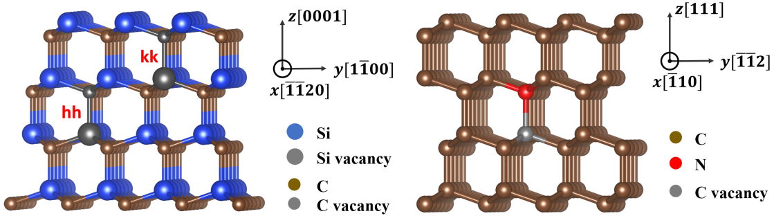
Figure 6.26: The structures of ( hh , kk )-VV in 4H-SiC (left) and NV in diamond (right). Lattices are slightly rotated around z axis to show more details.
