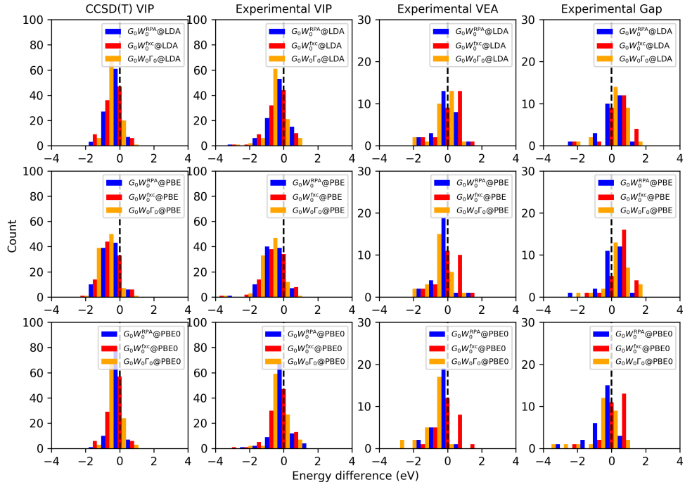
Figure 3.6: Vertical ionization potential (VIP), vertical electron affinity (VEA) and electronic gap of molecules in the GW100 set computed at G_0W_0^{\text{RPA}} , G_0W_0^{f_{\text{xc}}} and G_0W_0\Gamma_0 levels of theory, compared to experimental and CCSD(T) results (black dashed lines).
