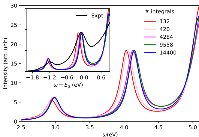
Figure 3.17: Optical absorption spectra of C_{60} in the gas phase computed by solving the BSE with several thresholds \xi for the screened exchange integrals. The resulting number of integrals is indicated. The inset shows the same spectra plotted as a function of \omega - E_g , and compared with experiment [176]. E_g is the electronic gap. Note that an accurate spectrum is obtained when using 4,284 integrals instead of the total number which is more than three times larger (14,400).
