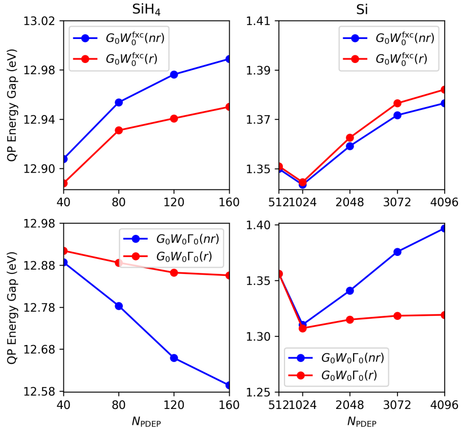
Figure 3.15: Convergence of GW quasiparticle gaps of \text{SiH}_4 and \text{Si} as a function of N_{\text{PDEP}} , using either un-renormalized (nr) or renormalized (r) \tilde{f}_{xc} matrices.
