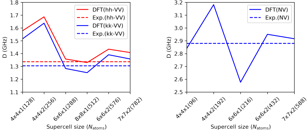
Figure 6.27: D value ( \frac{1}{2}(D_{xx} + D_{yy}) - D_{zz} ) for VV in 4H-SiC (left) and NV in diamond (right) as functions of supercell sizes. Calculations are done without strain and thus all defects have C_{3v} symmetry. E values ( \frac{1}{2}(D_{xx} - D_{yy}) ) are smaller than 2 MHz for all calculations.
