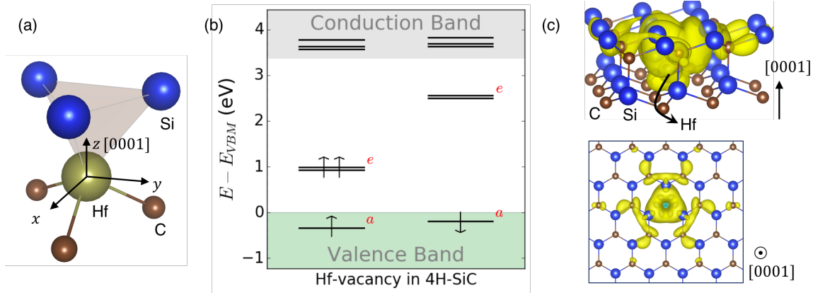
Figure 6.1: Hf-vacancy complex in 4H-SiC. (a) Proposed defect structure of a Hf-vacancy complex in 4H-SiC with (hh) axial configuration and C_{3v} symmetry: Hf substitutes Si at an h-site and it pairs with a C vacancy at the nearest neighboring h-site. Only the nearest neighboring Si and C atoms are shown for clarity. (b) The defect level diagram of the Hf-vacancy complex calculated at the DFT- DDH hybrid level of theory. The totally symmetric a state is located at -0.34 eV and -0.19 eV below the valence band edge in the spin-up and the spin-down channel, respectively. (c) Side (up) and top (down) views of the ground-state spin density of the Hf-vacancy defect calculated at the DDH level of theory.
