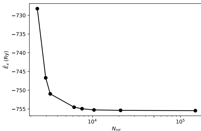
Figure 3.22: The Fock energy, \tilde{E}_x , as a function of the number of screened exchange integrals ( N_{int} ), for the ice model used in this work.
