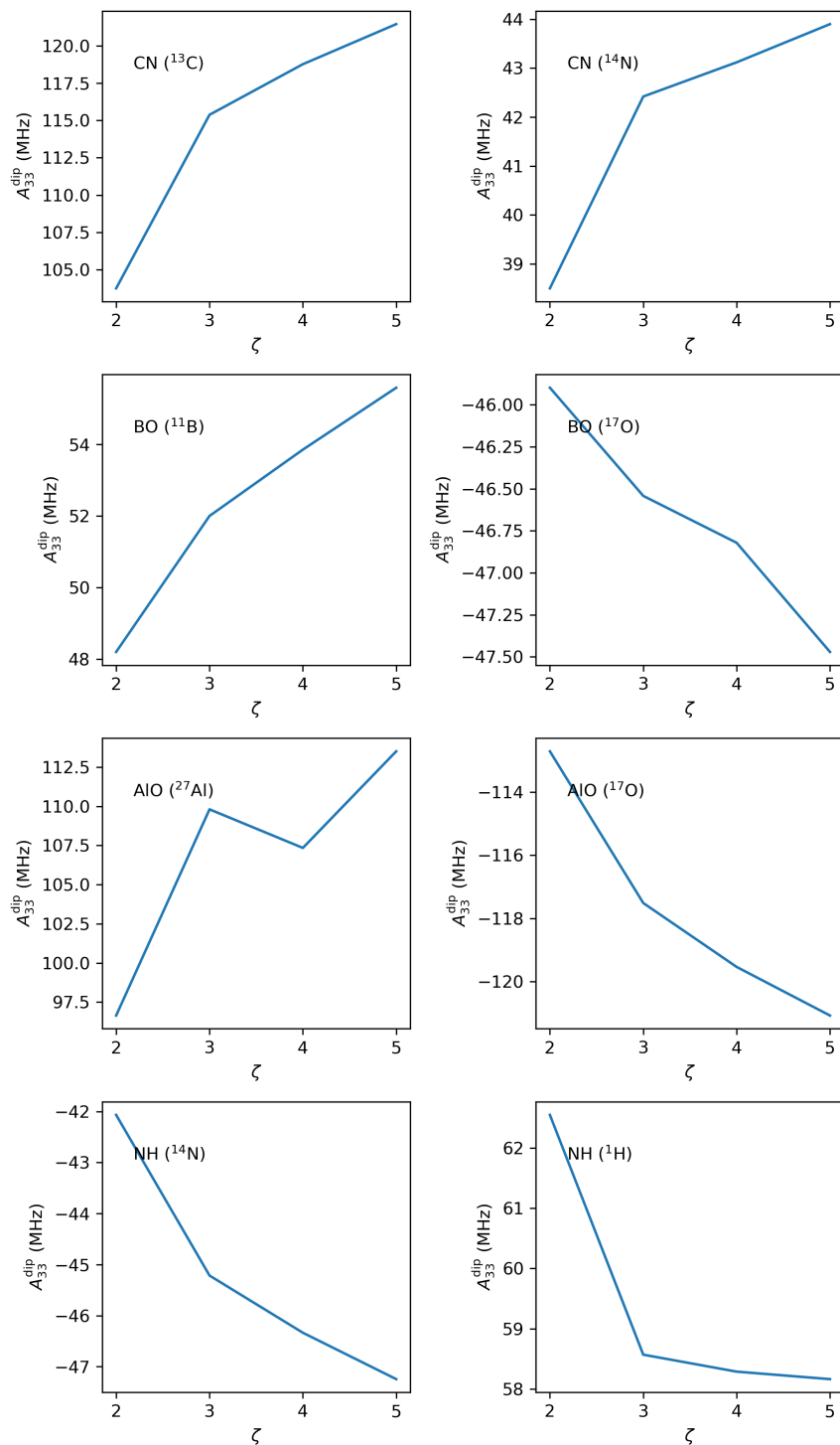
Figure 5.2: A_{33}^{\text{dip}} as a function of basis set.
