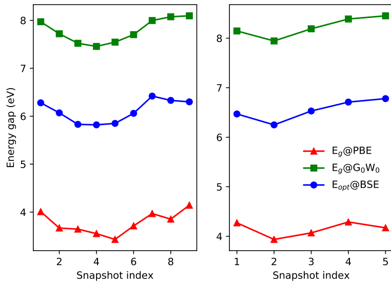
Figure 3.24: The BSE optical ( E_{opt} ) gap and the electronic ( E_g ) gaps computed with PBE and G_0W_0@PBE for different snapshots extracted from PIMD simulations with the MBPol potential (left-panel) and FPMD with the PBE functional (right-panel).
