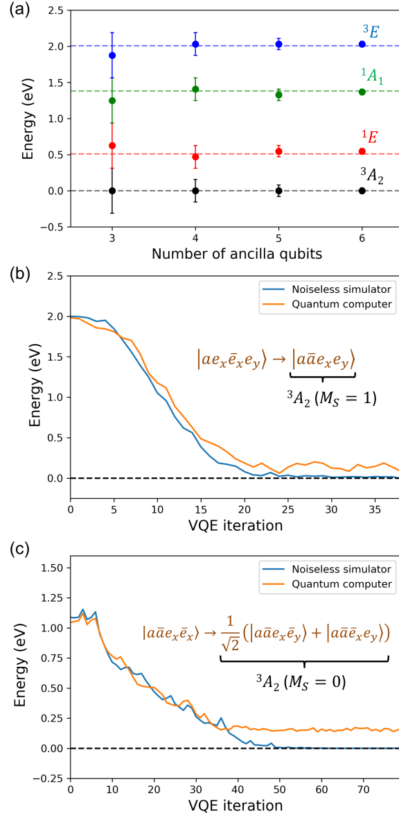
Figure 4.4: Quantum simulations of a minimum model of the NV center in diamond using the phase estimation algorithm (PEA) and a variational quantum eigensolver (VQE). The energy of the {}^3A_2 ground state manifold is set to zero for convenience. (a) PEA estimation of ground and excited states of the NV center. Error bars represent the uncertainties due to the finite number of ancilla qubits used in the simulations; dashed lines show classical FCI results. (b) VQE estimation of ground state energy, starting from |ae_x \bar{e}_x e_y\rangle state ( M_S = 1 ). (c) VQE estimation of ground state energy, starting from |a\bar{a}e_x \bar{e}_x\rangle state ( M_S = 0 ); strongly-correlated \frac{1}{2}(|a\bar{a}e_x \bar{e}_y\rangle + |a\bar{a}\bar{e}_x e_y\rangle) state ( M_S = 0 state in the {}^3A_2 manifold) is obtained with VQE.
