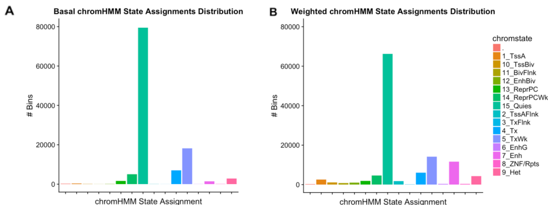
Figure 2.24: S17. Using a weighting scheme for chromHMM annotations increases the proportion of transcriptional and enhancer-like annotations. (A) Histogram showing the number of Hi-C loci (y-axis) assigned to each chromHMM annotation (x-axis) using maximum base pair overlap to assign each locus to a state. In the legend, '.' denotes that no annotation was found for a given bin. (TssA-Active TSS, TSSBiv-Bivalent/Poised TSS, BivFlnk-Flanking Bivalent TSS/Enh, EnhBiv-Bivalent Enhancer, ReprPC-Repressed PolyComb, ReprPCWk-Weak Repressed PolyComb, Quies-Quiescent/Low, TssAFlnk-Flanking Active TSS, TxFlnk-Transcription at gene 5' and 3', Tx-Strong transcription, TxWk-Weak transcription, EnhG-Genic Enhancers, Enh-Enhancers, ZNF/Rpts-ZNF genes and repeats, Het-Heterochromatin). (B) Same as A, only here, we assigned annotations after weighting chromHMM elements' overlaps with Hi-C loci by the reciprocal of their mean overlap in all our loci. This approach increases the number of 10kb Hi-C bins that are assigned to chromHMM annotations associated with transcriptional and enhancer activity (i.e. TssA, TssBiv, TssAFlnk, EnhG, Enh).
