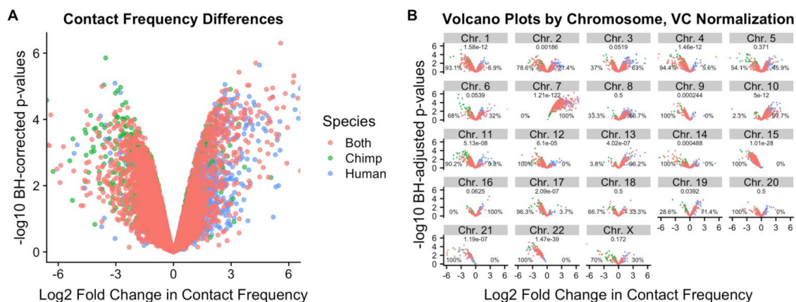
Figure 2.9: S2. Linear modeling reveals large-scale chromosomal differences in contact frequency, Juicer. (A) Volcano plot of \log_2 fold change in contact frequency between humans and chimpanzees (x-axis) against Benjamini-Hochberg FDR (y-axis), after filtering non-orthologous regions. Data are colored by the species in which the contact was originally identified as significant. (B) Per-chromosome volcano plot using the same legend as in A. P-values provided for a binomial test of the null that inter-species differences in contact frequencies are evenly distributed. The percentage of contacts with significant higher frequency in each species is noted. Of note is that many of the same chromosomal asymmetries in contact strength observed here are in the same chromosomes as those observed in the HOMER-normalized data (Fig 2.2).
