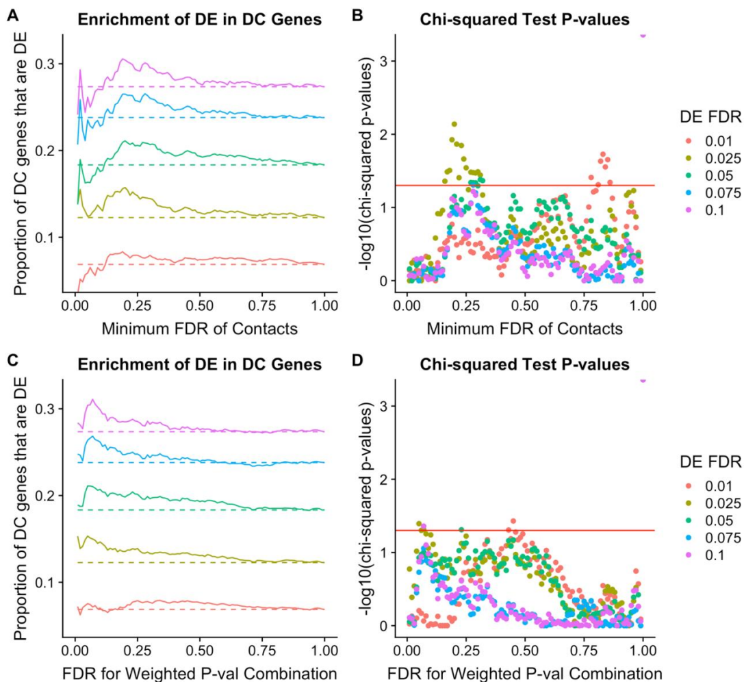
Figure 2.10: S3. Differentially expressed genes show enrichment for differential Hi-C contacts, Juicer. (A) Enrichment of inter-species differentially expressed (DE) genes with corresponding differences in Hi-C contact frequencies (DC) between the species. The proportion of DC genes that are significantly DE (y-axis) is shown across a range of DC FDRs (x-axis). Colors indicate different DE FDR thresholds, and dashed lines indicate the proportion of DE genes expected by chance alone. (B) P values of Chi-squared tests of the null that there is no difference in proportion of DE genes among DC genes (y-axis), shown for a range of DC FDRs (x-axis). In both panels, DC regions were chosen to have the minimum FDR supporting inter-species difference in contact frequency. (C) Same as A, but this time, a weighted p-value combination technique [189] was used to integrate each Hi-C bin's DC FDR across all of its contacts. (D) Same as B, but for the weighted p-value combination instead of the minimum FDR contact.
