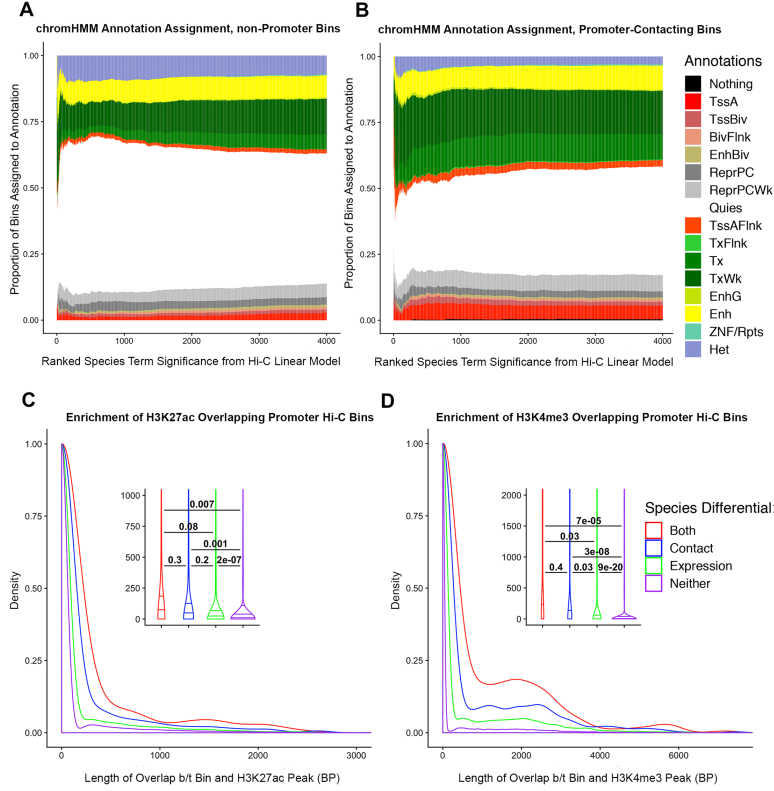
Figure 2.7: Overlap of epigenetic signatures and Hi-C contacts. (A) Hi-C loci that do not make contact with promoters are ranked in order of decreasing DC FDR (x-axis). The y-axis shows cumulative proportion of chromHMM annotation assignments for all Hi-C loci at the given FDR or lower. (TssA-Active TSS, TSSBiv-Bivalent/Poised TSS, BivFlnk-Flanking Bivalent TSS/Enh, EnhBiv-Bivalent Enhancer, ReprPC-Repressed PolyComb, ReprPCWk-Weak Repressed PolyComb, Quies-Quiescent/Low, TssAFlnk-Flanking Active TSS, TxFlnk-Transcription at gene 5' and 3', Tx-Strong transcription, TxWk-Weak transcription, EnhG-Genic Enhancers, Enh-Enhancers, ZNF/Rpts-ZNF genes and repeats, Het-Heterochromatin). (B) Same as A, but only considering Hi-C loci making contact with promoter bins. Results of separating promoter-contacting bins between DE and non-DE genes can be seen in 2.26 Fig. (C) Density plot of the base pair overlap between different classes of Hi-C contact loci and H3K27ac. Histone mark data were obtained from ENCODE in experiments carried out in human iPSCs. We grouped contacts into 4 classes, indicated by color: those that show differential contact between species, those that show differential expression between species, those that show both, and those that show neither. We used pairwise t-tests to compare differences in the mean overlap among the four classes of Hi-C loci. (D) Same as C, but performed on H3K4me3 data obtained from ENCODE, collected in hESCs. Results with other histone marks can be seen in 2.25 Fig.
