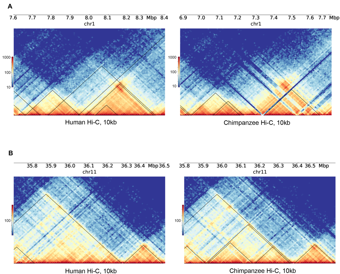
Figure 2.5: Examples of conserved and divergent TADs. (A) A region on chromosome 1 with examples of both conserved and divergent Arrowhead [74] TAD inferences (black lines). Both the larger TADs seen in the chimpanzee map (right) appear to be conserved in the human map (left), whereas several of the TADs inferred in the human map are noticeably absent from the chimpanzee map. (B) A region on chromosome 11, once again showing examples of conserved and divergent Arrowhead TAD inferences (black lines). All the TADs seen in the human map (left) appear conserved in the chimpanzee map (right), whereas three smaller TADs inferred in the chimpanzee map are not found in the human map, suggesting divergence.
