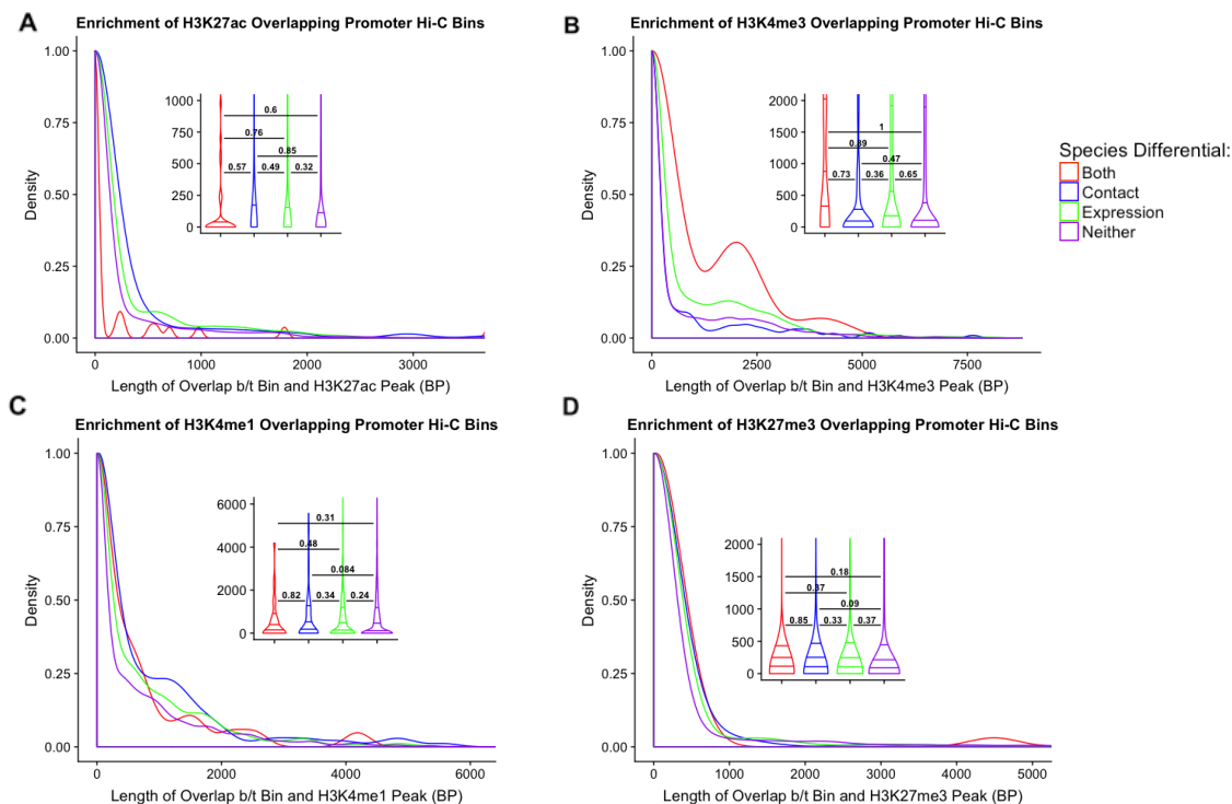
Figure 2.12: S5. Overlap of activating and repressive histone marks among Hi-C contacts, Juicer. (A) Density plot of the base pair overlap between different classes of Hi-C contact loci and H3K27ac. Histone mark data were obtained from ENCODE in experiments carried out in human iPSCs. We grouped contacts into 4 classes, indicated by color: those that show differential contact between species, those that show differential expression between species, those that show both, and those that show neither. We used pairwise t-tests to compare differences in the mean overlap among the four classes of Hi-C loci. Unlike in the HOMER-normalized data, we do not observe statistically significant differences in overlaps with H3K27ac between different locus classes. This may reflect the previous observation that the hiccups algorithm for assigning statistical significance of loops in Hi-C data is much more conservative than HOMER’s significance calling method [89]. (B) Same as A, but performed on H3K4me3 data obtained from ENCODE, collected in hESCs. (C) Same as A and B, but performed on H3K4me1 data obtained from ENCODE, collected in human iPSCs. (D) Same as A, B, and C, but performed on H3K27me3 data obtained from ENCODE, collected in human iPSCs.
