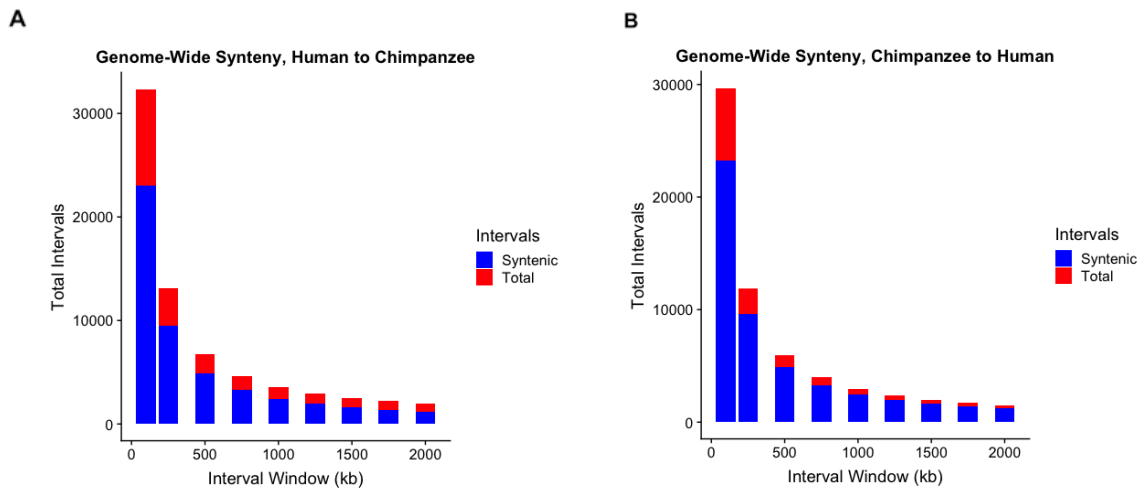
Figure 2.18: S11. Synteny of large scale linear genomic intervals between human and chimpanzee. (A) Across different window sizes (x-axis) for a genome-wide tiling of hg38, we plotted the number of total and syntenic linear intervals (y-axis), identified using the reciprocal best hits liftOver method [300, 140] we employed throughout the paper. (B) Same as A, but for a genome-wide tiling of panTro5.
