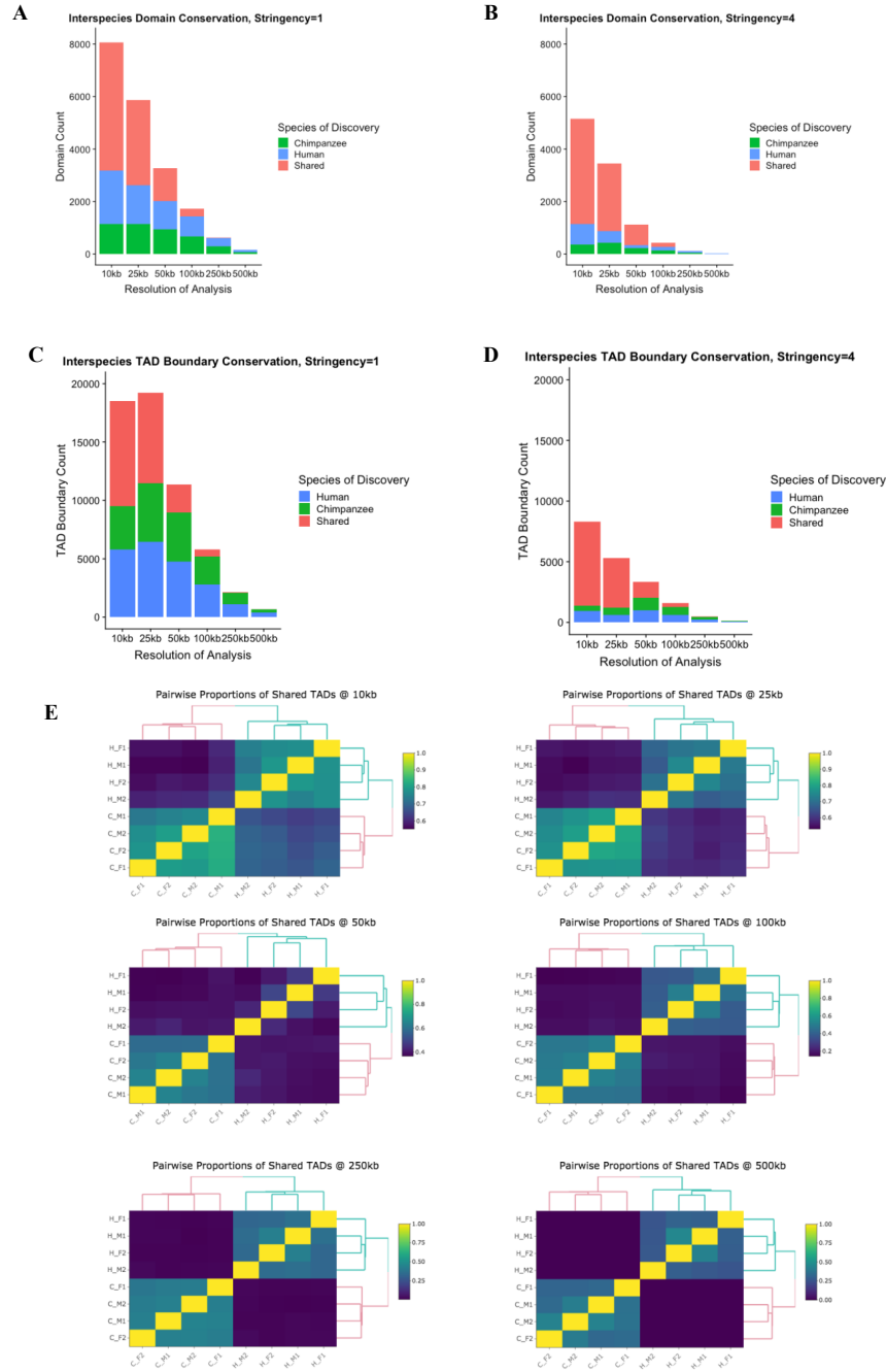
Figure 2.19: S12. Higher-order chromosomal structure in humans and chimpanzees with alternative analysis choices. (A) Across different resolutions (x-axis), we plotted the number of shared and species-specific domains (y-axis) identified with Arrowhead [74] on Juicer VC-normalized Hi-C maps from each individual. We called domain conservation here based on the method of Rao et al. [233] (highly similar results were observed with our 90% reciprocal overlap method, described in the text and available in the github repository associated with the paper)...(continued on next page)
