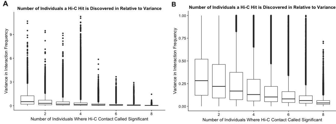
Figure 2.14: S7. Variance in interaction frequency as a function of the number of individuals in which a significant interaction is independently discovered. (A) Boxplots of variance in contact frequency across all 8 individuals on the y-axis, binned by the number of individuals in which an interaction is independently called significant on the x-axis. (B) Same as A, but zoomed in on the y-axis to visualize finer-scale variation.
