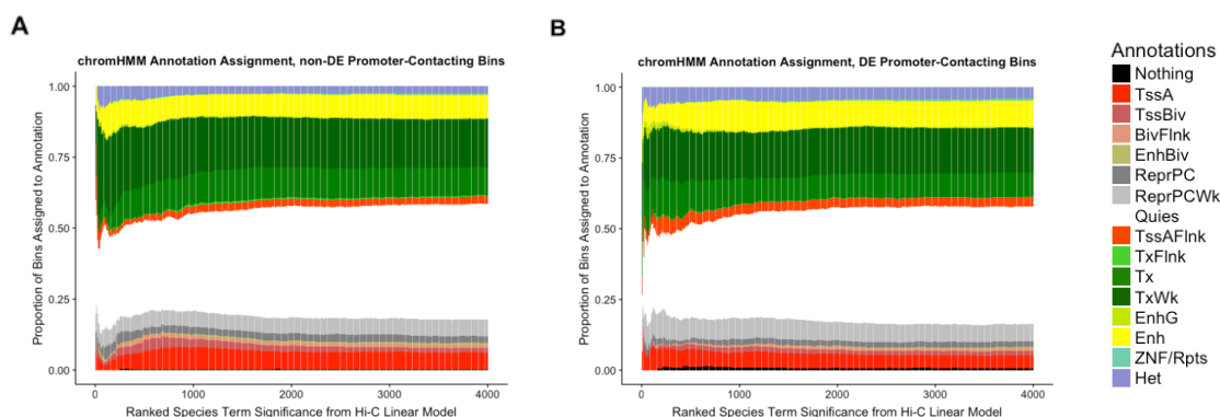
Figure 2.26: S19. Dynamics of chromHMM state among significant Hi-C contacts overlapping DE or non-DE genes. (A) Hi-C loci that make contact with promoters of genes that are not differentially expressed (DE) across species are ranked in order of decreasing DC FDR (x-axis). The y-axis shows cumulative proportion of chromHMM annotation assignments for all Hi-C loci at the given FDR or lower. (TssA-Active TSS, TssBiv-Bivalent/Poised TSS, BivFlnk-Flanking Bivalent TSS/Enh, EnhBiv-Bivalent Enhancer, ReprPC-Repressed PolyComb, ReprPCWk-Weak Repressed PolyComb, Quies-Quiescent/Low, TssAFlnk-Flanking Active TSS, TxFlnk-Transcription at gene 5' and 3', Tx-Strong transcription, TxWk-Weak transcription, EnhG-Genic Enhancers, Enh-Enhancers, ZNF/Rpts-ZNF genes and repeats, Het-Heterochromatin). (B) Same as A, but only considering Hi-C loci making contact with promoters of genes that are differentially expressed (DE).
