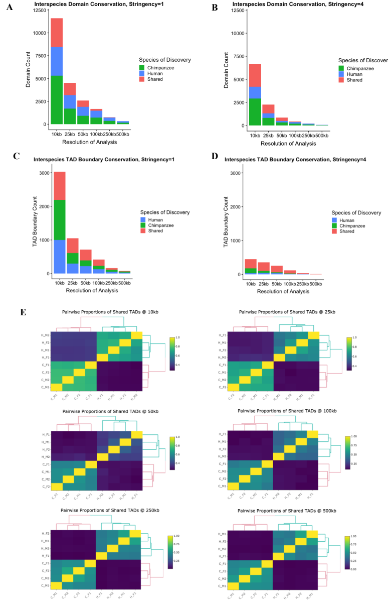
Figure 2.21: S14. Higher-order chromosomal structure in humans and chimpanzees with alternative algorithms (TopDom). (A) Across different resolutions (x-axis), we plotted the number of shared and species-specific domains (y-axis) identified with TopDom [261] on HOMER-normalized Hi-C maps from each individual. We called domain conservation here based on the method of Rao et al. [233] (highly similar results were observed with our 90% reciprocal overlap method, described in the text and available in the github repository associated with the paper)...(continued on next page)
