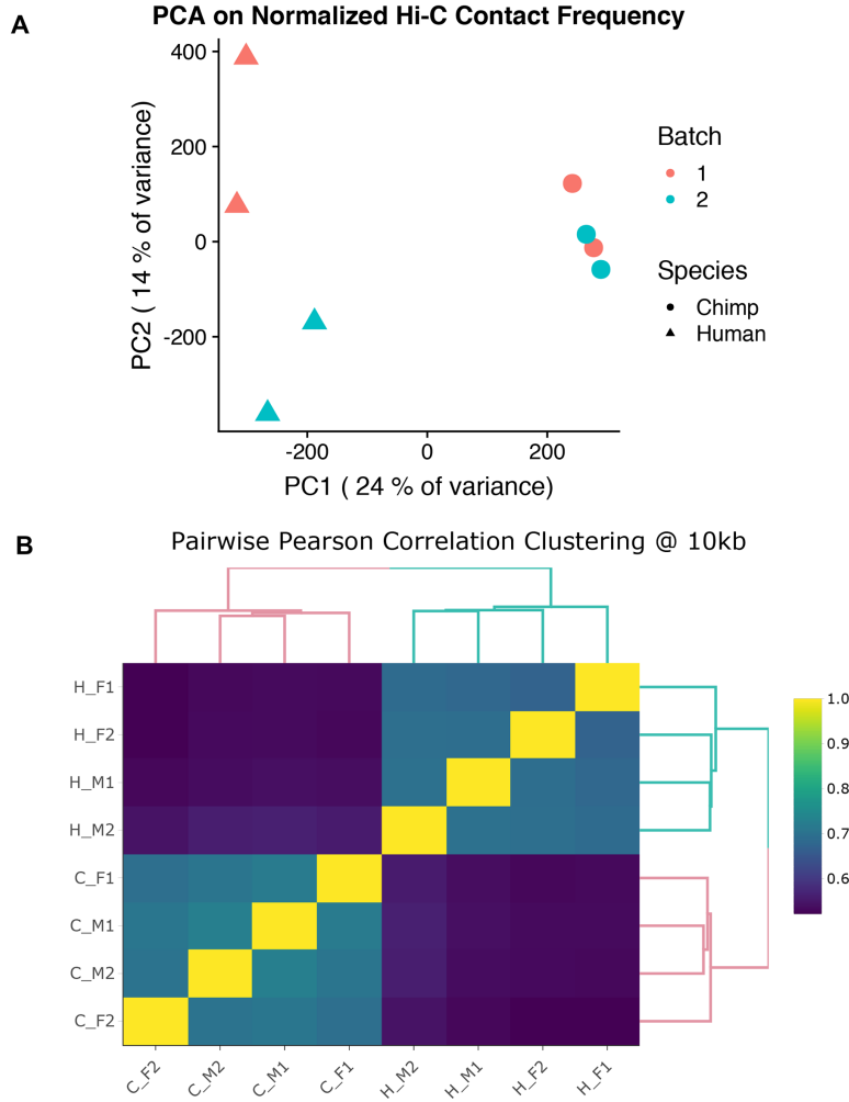
Figure 2.1: General patterns in Hi-C data. (A) Principal components analysis (PCA) of HOMER-normalized interaction frequencies for the union of all contacts in humans (triangles) and chimpanzees (circles). PC1 is highly correlated with species ( r = 0.98 ; P < 10^{-5} ). (B) Unsupervised hierarchical clustering of the pairwise correlations (Pearson's r^2 ) of HOMER-normalized interaction frequencies at 10 kb resolution. The first letter in the labels demarcates the species (H for human and C for chimpanzee), and the following symbols indicate sex (male, M or female, F) and batch (1 or 2).
