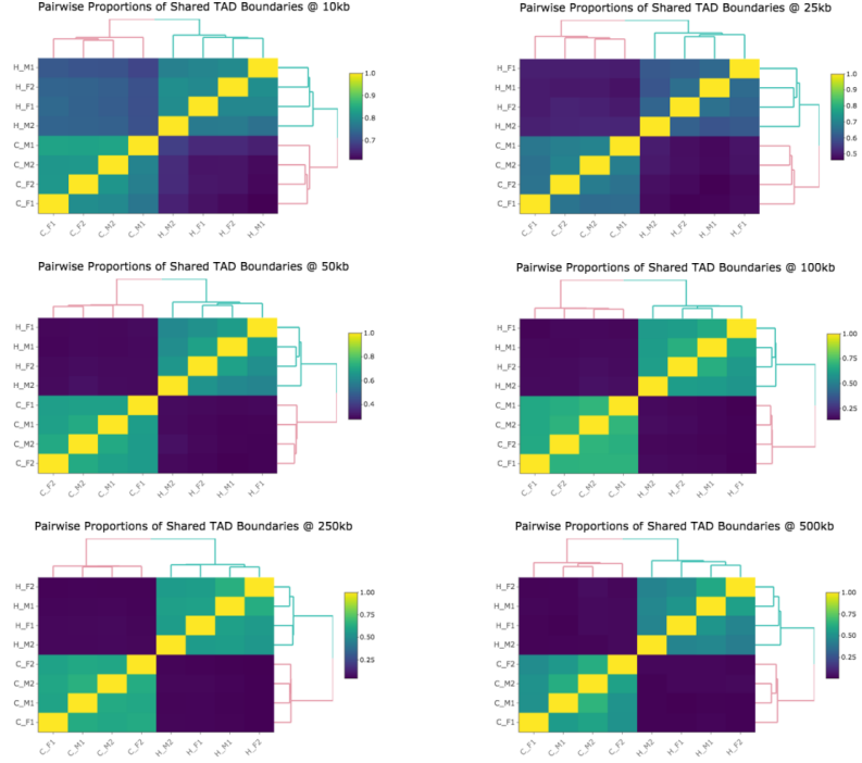
Figure 2.19: (continued from previous page) Domain count values represent the average interspecies sharing across all individuals, with no filtering for domain robustness (that is, assessing all domains discovered and orthologously mappable). Under this analysis paradigm we observe relatively low sharing across species ( \sim 60\% at 10kb). (B) Same as A, but this time, only considering TADs that were found across all 4 individuals within either one of the species (fixed TADs). Restricting to this subset increases the percentage of conservation to 78%, although the set of TADs being examined is much smaller. (C) Same as A, but for boundaries instead of domains. Boundaries were defined as 15kb flanking regions at the edges of inferred Arrowhead domains. Because the TADs called by Arrowhead are nested, we merged boundaries here to obtain unique genomic intervals, rather than counting boundaries repeatedly. We then considered boundaries shared between individuals if they had any overlap. (D) Same as B, but for boundaries instead of domains (i.e. considering only boundaries fixed within species). Here, the highest estimate of conservation we obtain is 83% of boundaries conserved across species at 10kb resolution. (E) Unsupervised hierarchical clustering of the pairwise proportions of shared TADs between all individuals in our study at a variety of resolutions, using the Rao et al. [233] methodology for calling conservation. The first letter in the labels demarcates the species (H for human and C for chimpanzee), and the following symbols indicate sex (male, M or female, F) and batch (1 or 2). Heatmaps are not necessarily symmetric because different numbers of TADs were discovered in different individuals; rows represent an individual's shared proportion of TADs (individual total) with each other individual. Highly similar clustering results were observed when using our domain conservation calling paradigm (shown in github repository associated with paper). (F) Same as E, but for boundaries instead of domains.
