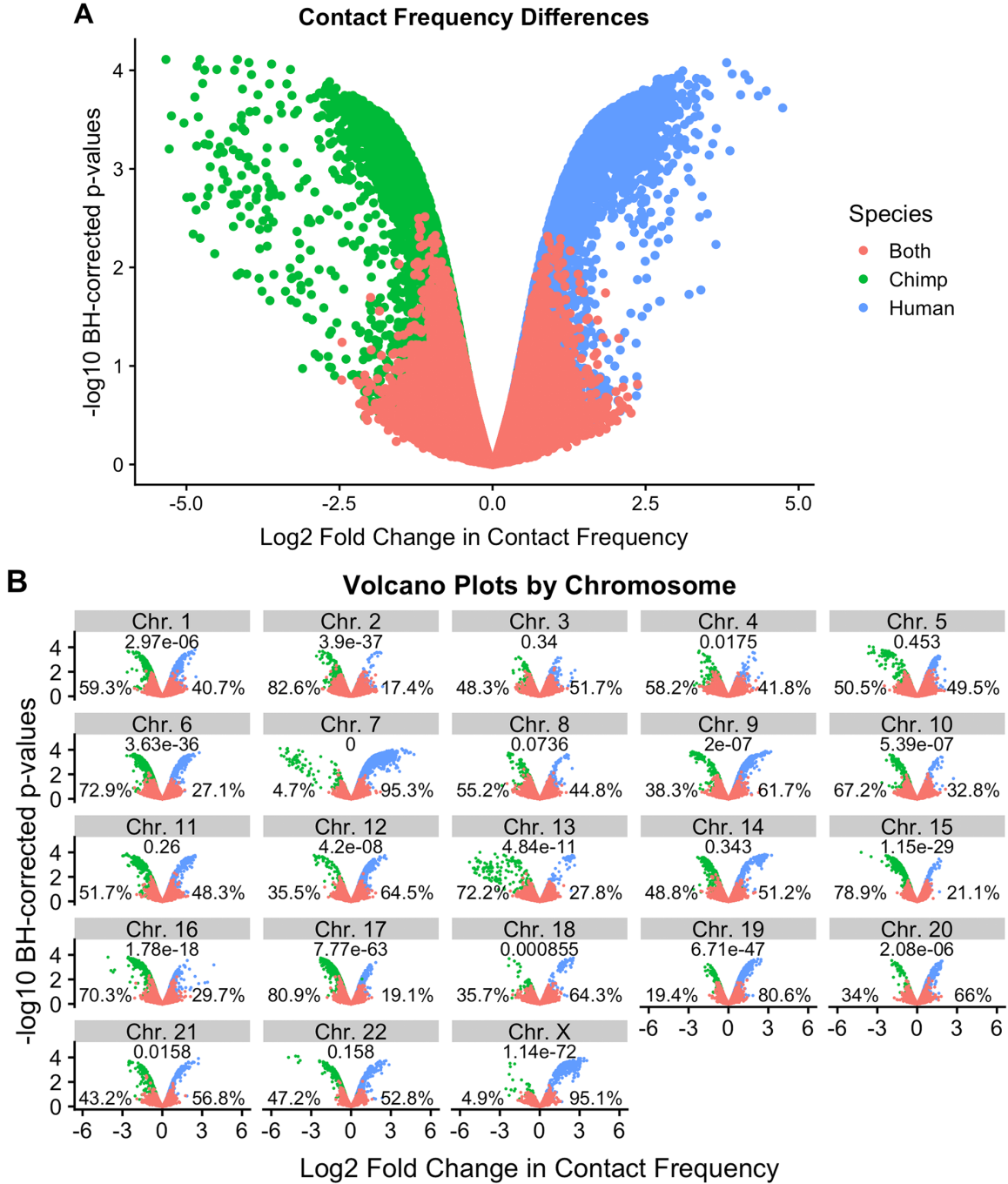
Figure 2.2: Linear modeling reveals large-scale chromosomal differences in contact frequency. (A) Volcano plot of \log_2 fold change in contact frequency between humans and chimpanzees (x-axis) against Benjamini-Hochberg FDR (y-axis), after filtering non-orthologous regions (results for unfiltered data are plotted in S9 Fig). Data are colored by the species in which the contact was originally identified as significant. (B) Per-chromosome volcano plot using the same legend as in A. P-values provided for a binomial test of the null that inter-species differences in contact frequencies are evenly distributed. The percentage of contacts with significant higher frequency in each species is noted.
