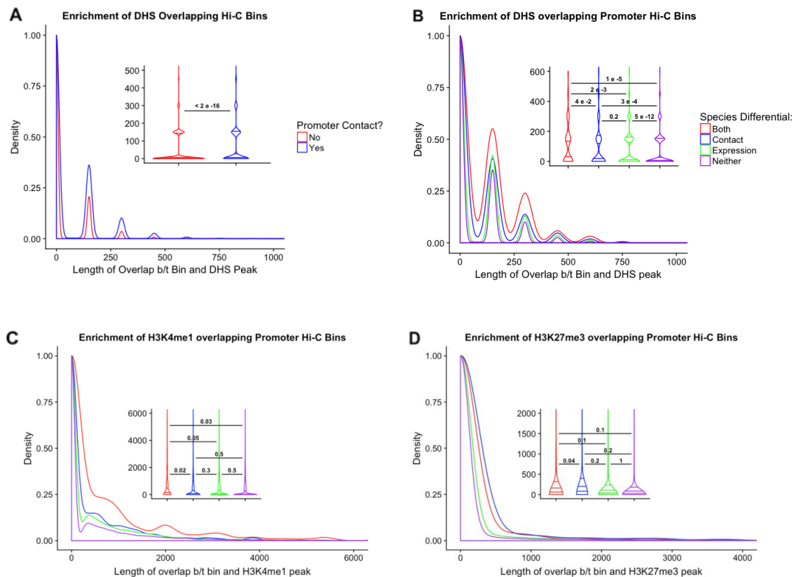
Figure 2.25: S18. Overlap of epigenetic signatures and Hi-C contacts. (A) Density distribution of the base pair overlap between DHS peaks downloaded from ENCODE and our Hi-C loci. Plot is split between Hi-C loci that contact a promoter and those that do not. Inlay is a violin plot of the same distributions, with lines and numbers indicating pairwise t-tests of the mean, and their corresponding significance levels. (B) Density plot similar to A, but only considering Hi-C loci involved in contact with a promoter, and separating contacts into 4 classes, indicated by color: those that show differential contact between species, those that show differential expression between species, those that show both, and those that show neither. We used pairwise t-tests to compare differences in the mean overlap among the four classes of Hi-C loci. (C) Same as in B, but for the active histone mark H3K4me1. (D) Same as in B and C, but for the repressive histone mark H3K27me3.
