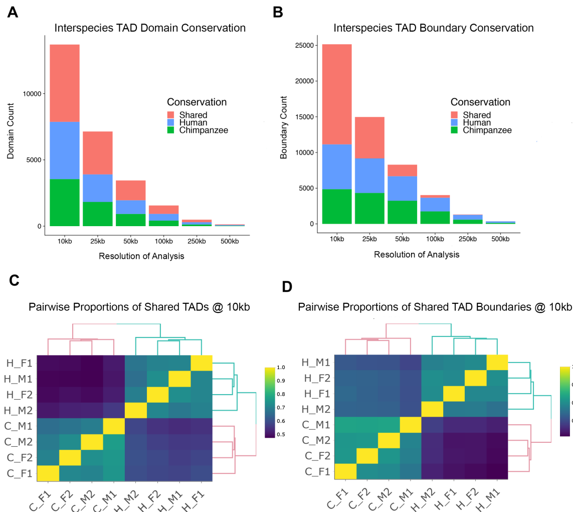
Figure 2.4: Higher-order chromosomal structure in humans and chimpanzees. (A) Across different resolutions (x-axis), we plotted the number of shared and species-specific domains (y-axis) identified with Arrowhead [74] using the consensus map from each species (alternative approaches plotted in 2.19–2.21 Figs). (B) Same as A, but for TAD boundaries instead of the domains themselves. Boundaries were defined as 15kb flanking regions at the edges of inferred Arrowhead domains. (C) Unsupervised hierarchical clustering of pairwise comparison of TADs across all individuals. These proportions were obtained using Arrowhead TAD inferences on each individual at 10kb resolution. Proportions indicated by color scale on right. Similar plots using analysis at different resolution are available in 2.19 and 2.21 Figs. (D) Similar to C, but for TAD boundaries instead of the domains themselves.
