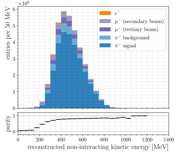
(b) Reconstructed kinetic energy of non-interacting hits along with selection purity p_{\text{non-int}}^{\text{MC}}
