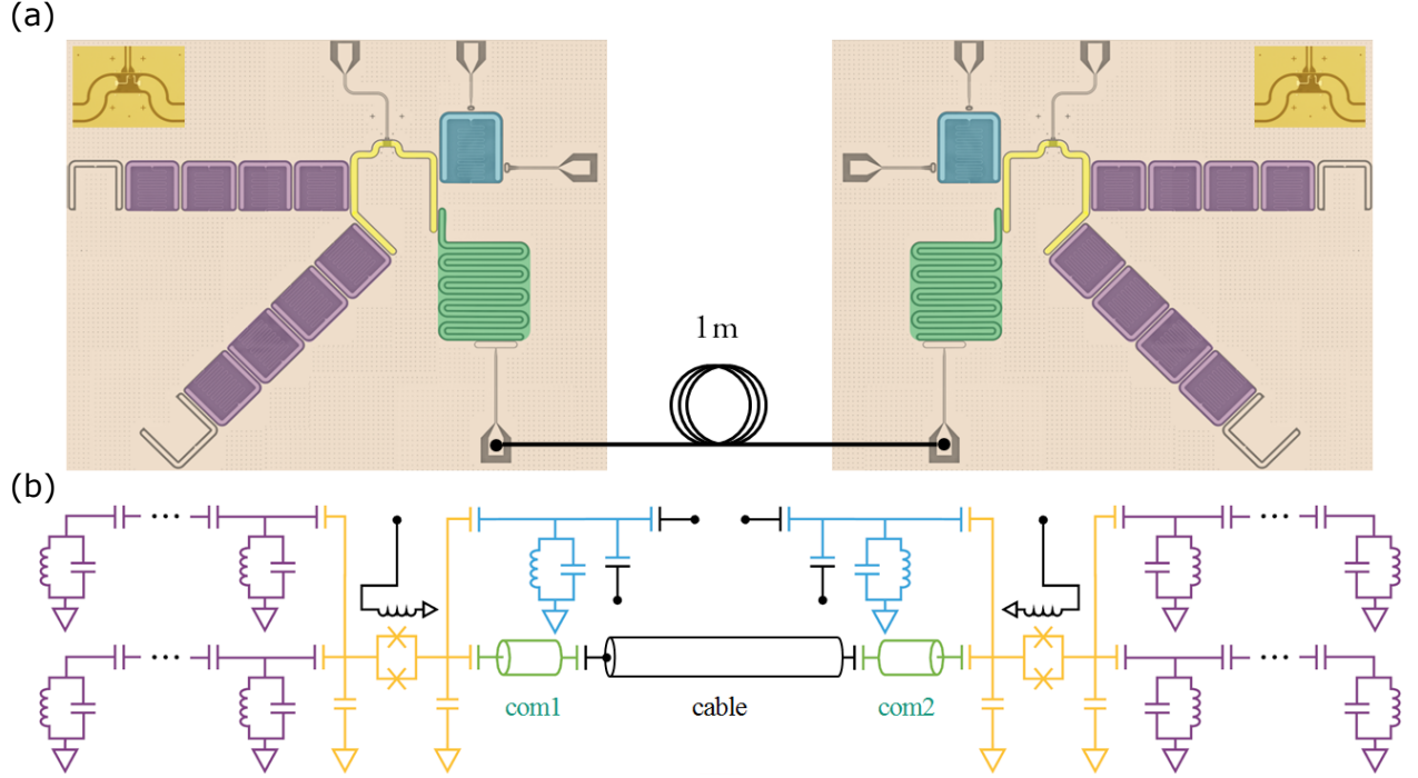
Figure 3.5: The communication network comprised of two modules connected by a coaxial cable. (a, b) False-colored photo and circuit diagram of the communication network. The two chips are connected by a \sim 1 m long, Tin-dipped Hand-formable Microwave Cable (UT-085C-Form) with silver-plated copper wire, which is quite lossy and has a lifetime around 50 ns. Without using a circulator along the communication channel, this creates a reciprocal network that allows for bi-direction photonic communication between the two modules.
