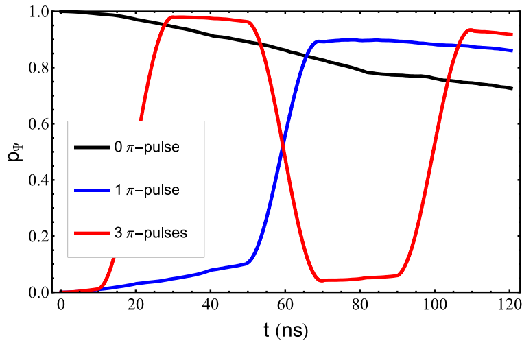
Figure 2.13: Monte Carlo wavefunction simulation of spin echo sequence under 1/f dephasing noise. Qubit is initialized at the equal superposition of the ground and excited state at the beginning of time. Under free evolution without spin echo, qubit decoheres according to the black line. A \pi pulse inserted in the middle of time flips the qubit, causing the phase to refocus under the autocorrelated 1/f noise and the increase of the decoherence time shown by the blue curve. Inserting more \pi pulses further suppresses the 1/f noise and leads to T_2 \rightarrow 2T_1 , shown by the red curve. The Gaussian rather than exponential decay envelope is indicative of the 1/f spectrum.
