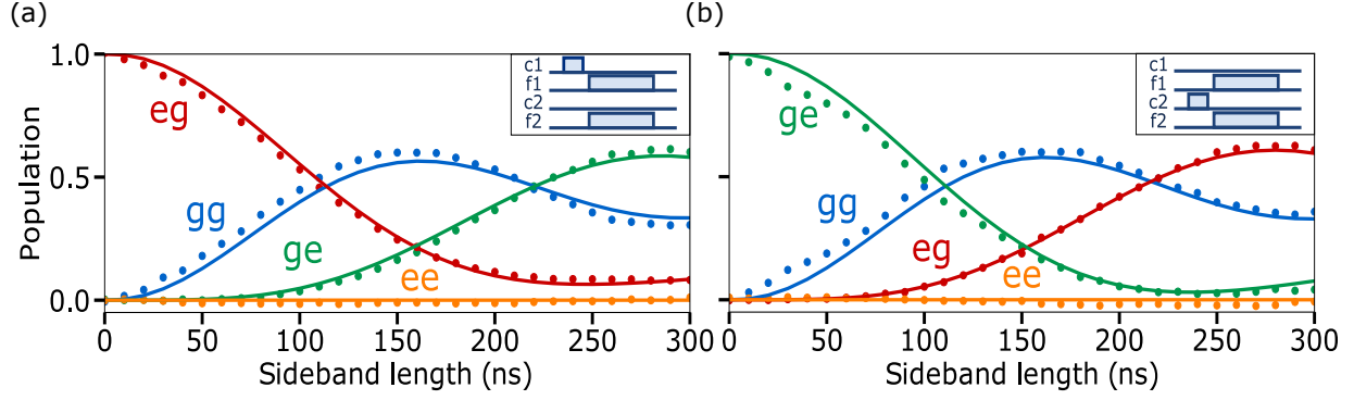
Figure 3.7: Bidirectional excitation transfer. The inset at top right shows the pulse sequence used to implement excitation transfer. The labels c1, c2 denote the charge drives on qubits 1 and 2, respectively, and f1, f2 the respective flux drives. We first apply a \pi pulse to excite one of the qubits, then simultaneously switch on the sideband flux pulse to drive the transfer process. Using the same sideband sequence, but instead applying the \pi pulse to the other qubit, we can send a single photon in the opposite direction. The transfer fidelity is limited by qubit dephasing and photon decay in the communication mode. Described in the following, the transfer process in different directions have slightly different loss mechanisms. (a) Excitation transfer from qubit 1 to qubit 2. Notice that in this transfer process the sender qubit is not able to fully receive its excitation (population of |eg\rangle does not reach zero). As confirmed by the master equation simulation, this is due to the dephasing of qubit 1. The remaining errors arise from communication cavity loss and dephasing of qubit 2, which is less than that of qubit 1. (b) Excitation transfer from qubit 2 to qubit 1. In this process, while qubit 2 releases most of its excitations (population of |ge\rangle comes close to zero), the dephasing of qubit 1 prevents it from capturing all the excitations in the communication mode, resulting in a slightly higher final population in |gg\rangle . The resulting fidelities for the transfer in the two directions are similar: \{P_{|ge\rangle}, P_{|eg\rangle}\} \approx 61\% , confirming the results from our numerical simulation.
