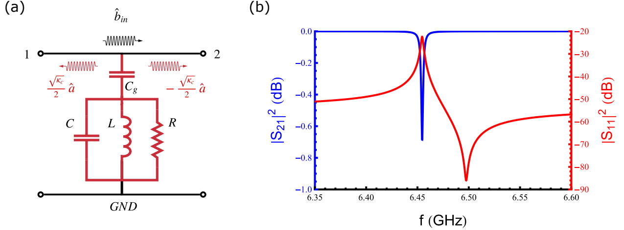
Figure 2.14: Quantum input-output theory of an RLC oscillator coupled to a “hanger” transmission line. (a) The cavity is driven by an input field \hat{b}_{\text{in}} propagating from port 1 to port 2, while the intra-cavity field \hat{a} leaks into the transmission line and propagates along both directions. The output fields detected at port 1 and port 2 are from the mixing between the input field and the intra-cavity field. (b) The transmission and the reflection coefficient as functions of the drive frequency. Hanger line readout allows the determination of the internal and coupling quality factors of the cavity from fitting the line-shapes with Eq. 2.143.
