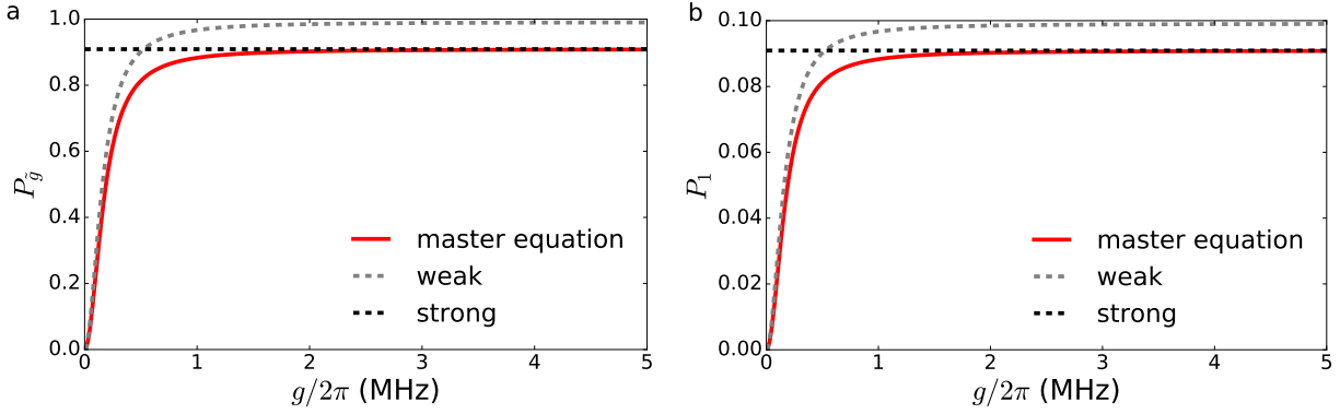
Figure 4.7: (a) The stabilized state population and (b) mean cavity photon number for stabilization angle \theta = \pi , as a function of the coupling strength g = \langle \tilde{e}0 | \hat{\mathcal{H}}_{int} | \tilde{g}1 \rangle , calculated with \kappa/2\pi = 1 MHz, \gamma/2\pi = 0.1 MHz, \gamma_\phi/2\pi = 0.1 MHz. Parameters are exaggerated for enhancing visual contrast and do not reflect experimental values. At \theta = \pi , the rotating frame ground state overlaps with the lab frame excited state, i.e. |\tilde{g}\rangle = |e\rangle . The exact solution from the master equation coincides with the weak coupling formula when g is small, whereas it falls into its asymptote predicted by the strong coupling formula when g is big, showing an good agreement between the theory and the numerical calculation.
