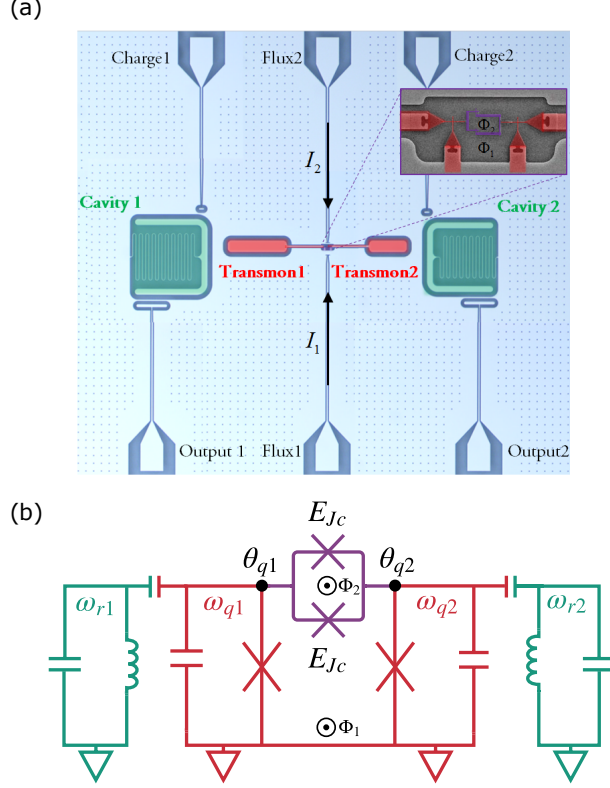
Figure 5.6: (a) False-colored circuit micrograph and (b) circuit diagram showing the VSLQ circuit components. The two transmons are plotted in red and will be used as logical qubits. In green are the two lumped-element resonators designed to be low-Q as the ancillary qubits, which are capacitively coupled to the transmons with fixed coupling strengths. At the heart of the device lies the dc-SQUID in purple, which, along with the transmon junctions, forms two superconducting loops controlled by tunable fluxes \Phi_1 and \Phi_2 , giving rise to the tunable nonlinear coupling term in Eq. 5.11, which is crucial for the generation of the VSLQ Hamiltonian.
