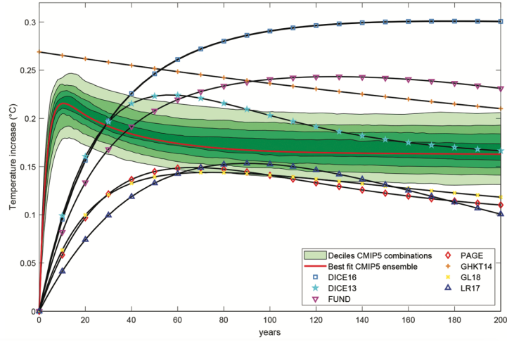
Figure 3.24: Pulse experiment: \mathcal{E} = 100 \text{ GtCO}_2 at t = 0 Comparison across different IAMs, Dietz et al. (2021)
