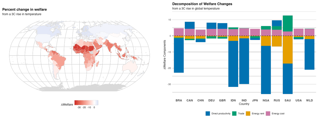
Figure 2.4: The welfare effects of a 3°C rise in global temperature.
