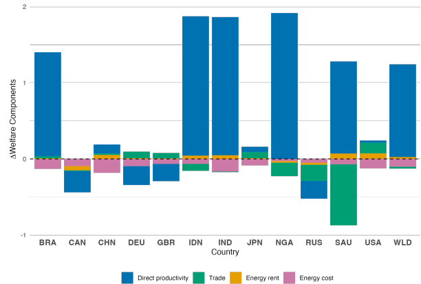
Decomposition of welfare changes from a $50/ton carbon tax in the US
