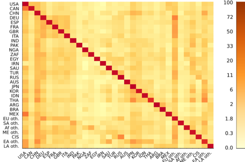
Figure 3.23: Trade shares as measured in Conte et al. (2022)
