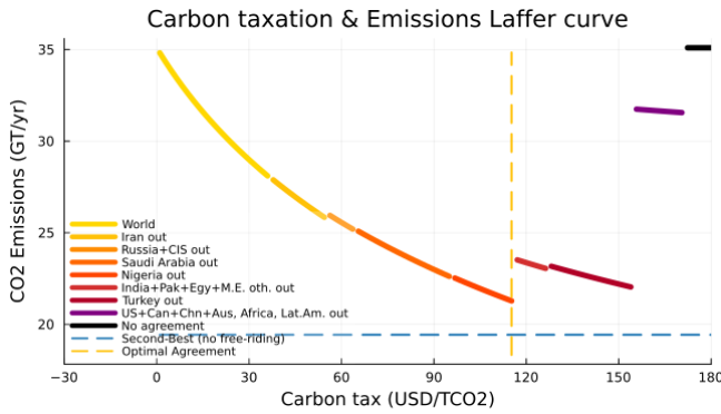
Figure 3.13: Global Emissions (yearly) for different carbon taxes a given tariff t^b = 50\%
