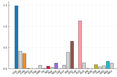
Figure 3.4: Oil-gas production, GTOE (gigatons oil equiv.), avg. 2018-2023
