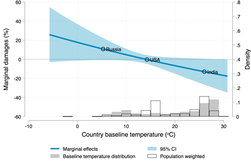
Figure 2.2: Marginal damages on productivity from a 1 degree change in local temperature versus country baseline temperature.
