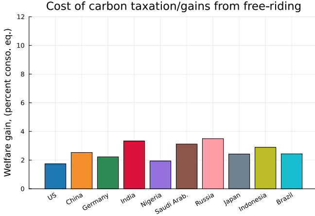
Figure 3.8: Welfare gain for country i of unilaterally deviating from a world agreement setting a $131 carbon tax
