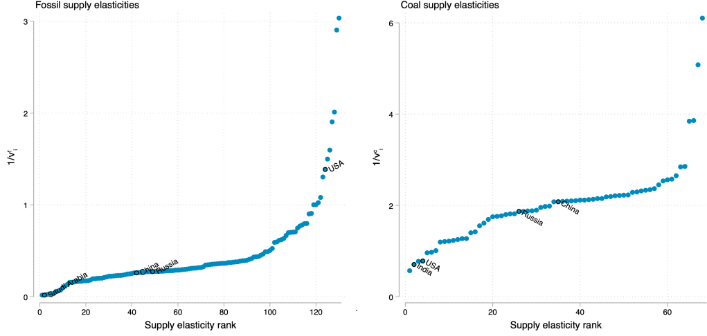
Figure 2.3: Empirical Bayes estimates of oil-gas and coal energy supply elasticities
