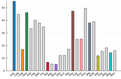
Figure 3.3: GDP per capita, Thsds 2011-USD PPP, avg. 2018-2023
