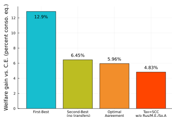
Figure 3.16: Global welfare (percent conso. eq.), comparison across equilibria
