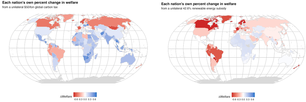
Figure 2.6: Left: each country's individual welfare change from pursuing unilateral carbon taxation. Right: each country's individual welfare change from pursuing a unilateral renewable subsidy.
