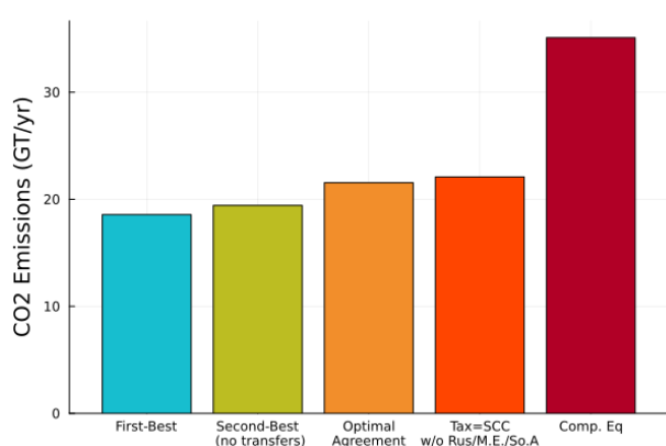
Figure 3.15: Global Emissions (yearly) comparison across equilibria
