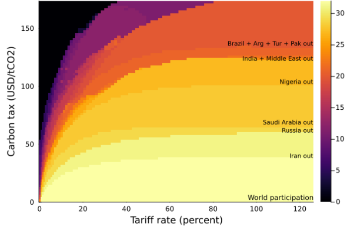
Figure 3.10: Participation: Intensive and extensive margin trade-off for agreement design: t^e on y-axis, t^b on x-axis
