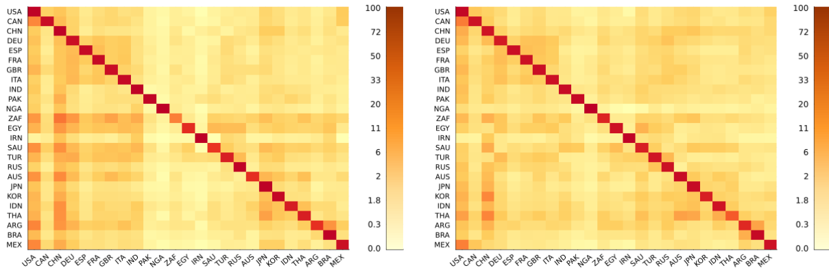
Figure 2.10: Left: Trade shares matrix, \mathbf{S} . Right: Income shares matrix \mathbf{T} . See main text for details.
