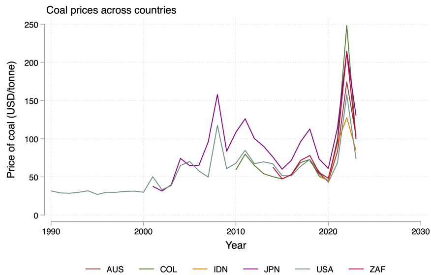
Figure 2.11: Coal prices in several countries.
