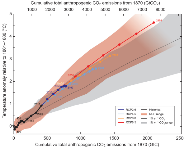
Figure 1.1: Linear temperature model - IPCC report
