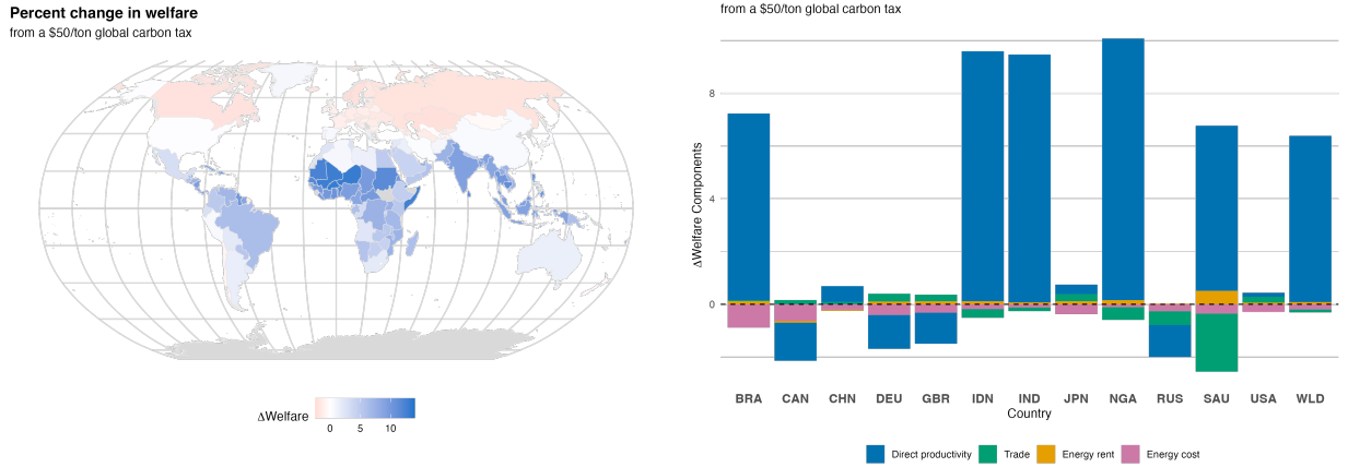
Figure 2.9: The welfare effects of a $50 carbon tax imposed in every country around the world.
