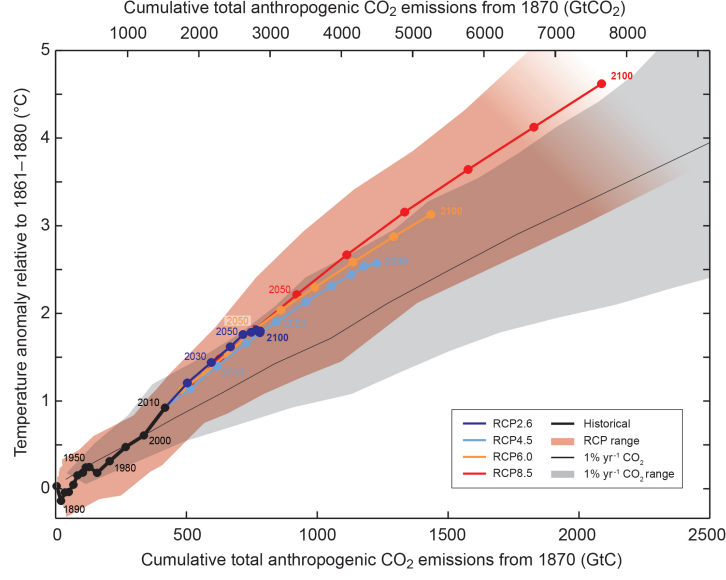
Figure 3.1: Linear temperature model – Cumulative emissions and temperature, IPCC et al. (2022)
