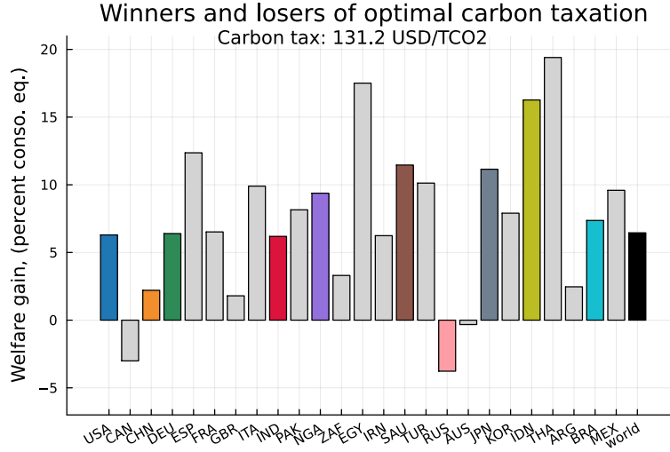
Figure 3.7: Welfare gains across countries – Second-Best equilibrium
