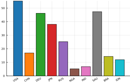
Figure 1.3: GDP per capita Thsds 2011-USD PPP, avg. 2018-2023
