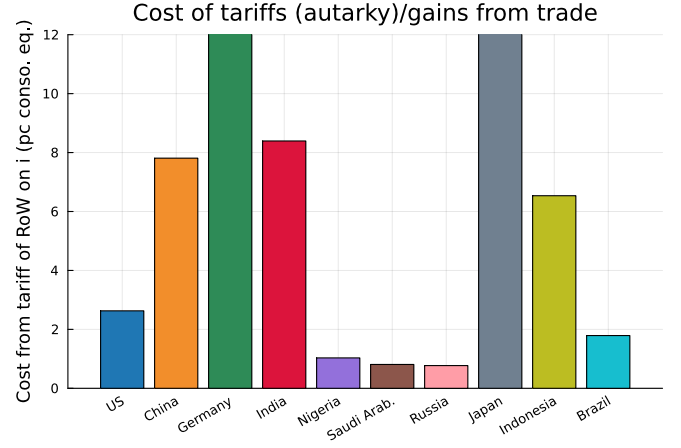
Figure 3.9: Losses for country i of country j \neq i imposing a 500% tariff on country i
