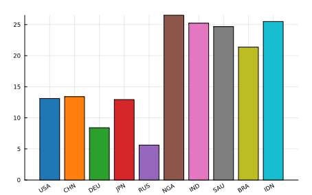
Figure 1.5: Temperatures avg. population-weighted 2015
