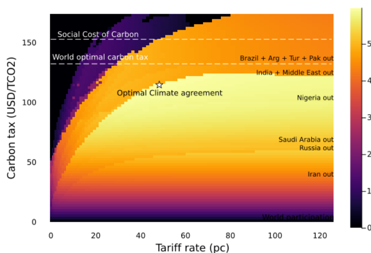
Figure 3.12: Welfare over different climate agreements t^e on y-axis, t^b on x-axis
