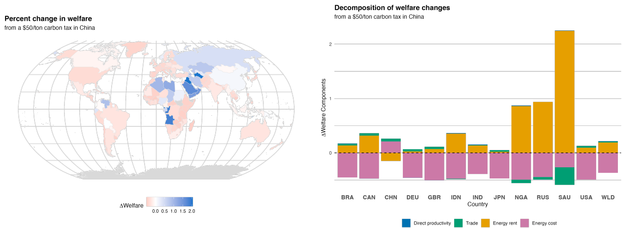
Figure 2.5: The welfare effects of a $50/ton carbon tax imposed unilaterally by China.
