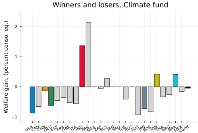
Figure 3.17: Welfare across countries Optimal climate fund: \alpha^{\varepsilon,\star} = 15\%
