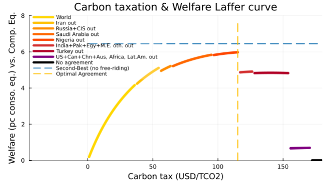
Figure 3.14: Global welfare (percent conso eq.), compared to Competitive Equilibrium for a given tariff t^b = 48\%
