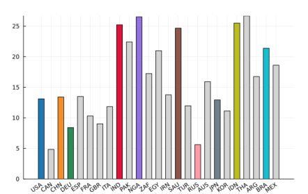
Figure 3.5: Temperature, Avg. pop-weighted, 2015
