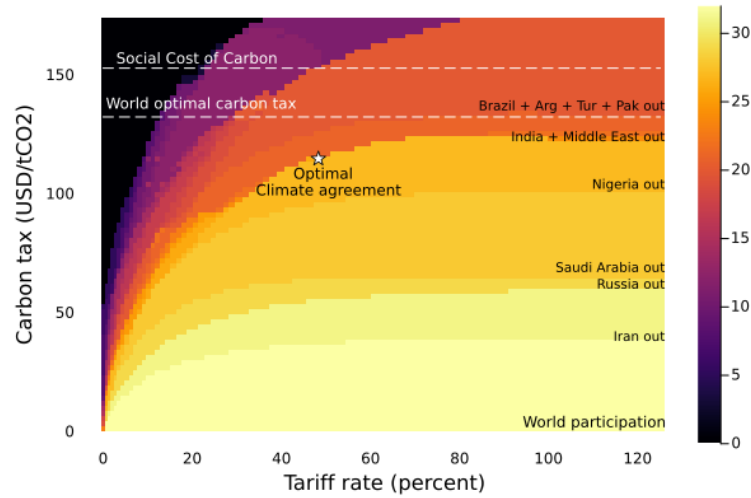
Figure 3.11: Optimal climate agreement: participation as function of t^e on y-axis and t^b on x-axis
