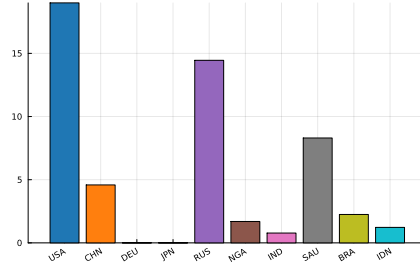
Figure 1.4: Oil-gas production GTOE (gigatons oil equiv.), avg. 2018-2023
