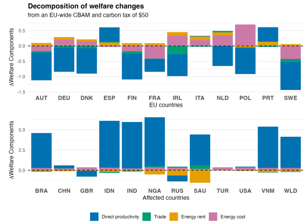
Figure 2.7: Left: changes in welfare from a EU climate club. Right: Decomposition of welfare changes within the EU (top) and for major trade partners and losers of climate change (bottom).
