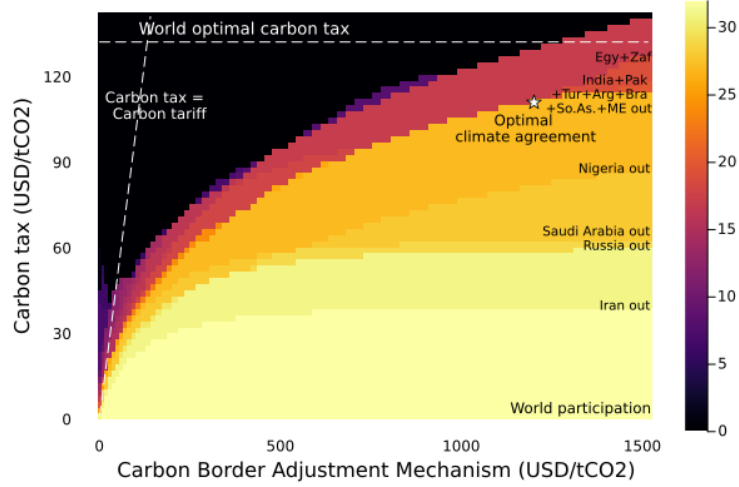
Figure 3.18: Agreement participation Penalty with carbon tariffs: t_{ij}^b = \xi_j^y t^{b,\varepsilon} (with t^{b,\varepsilon} on x-axis)
