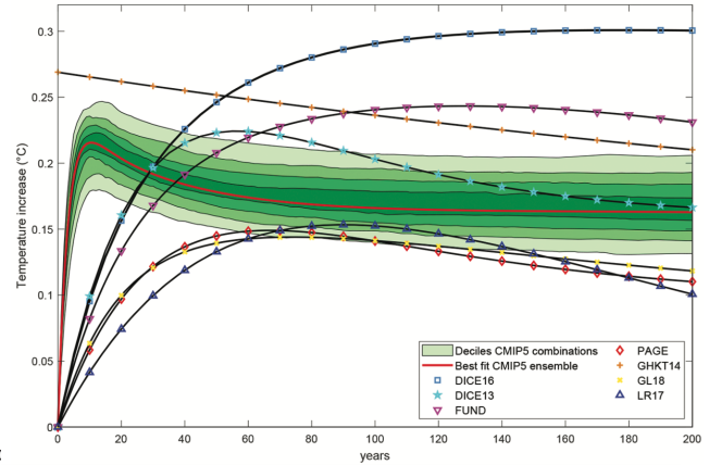
Figure 1.2: Pulse experiment, CMIP5 vs. IAMs
