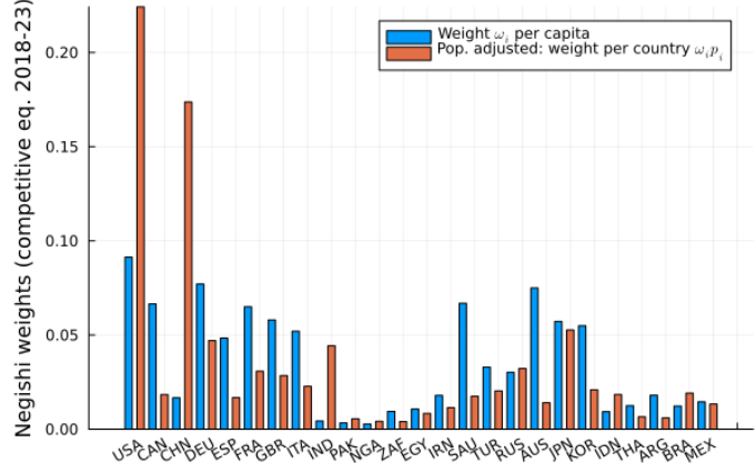
Figure 3.2: Pareto weights across regions weights \omega_i (blue, left), \hat{p}_i \omega_i (red, right)
