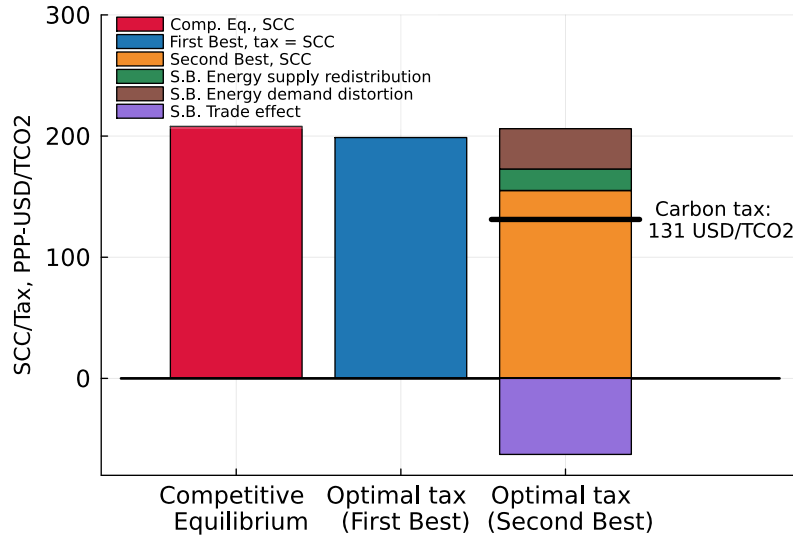
Figure 3.6: Social Cost of Carbon and optimal carbon taxation
