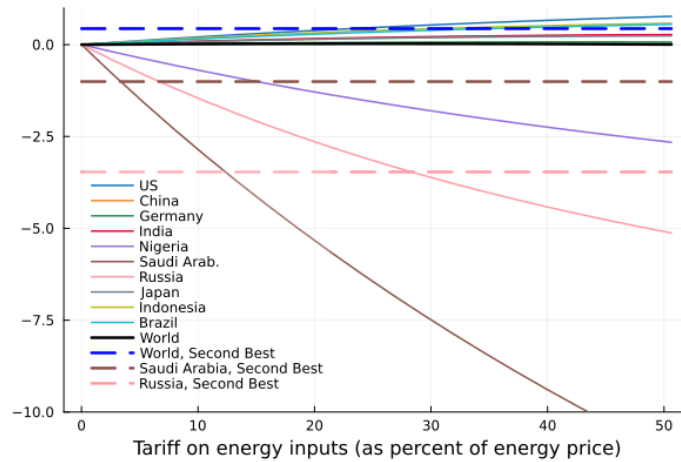
Figure 3.19: Welfare for world, large members, and non-members Tariff on oil-gas energy: t^{bf\star} = 40\%
