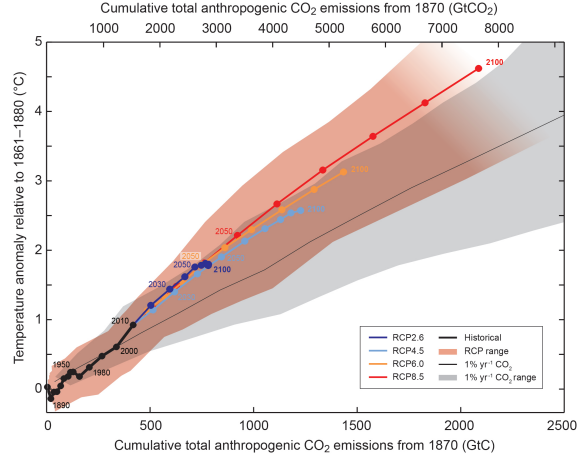
Figure 2.1: Cumulative emissions and temperature, IPCC et al. (2022)
