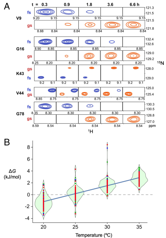
Fig. 2. The gsKaiB^{D91R} \rightleftharpoons fsKaiB^{D91R} equilibrium is sensitive to temperature. ( A ) A sample of 15 N-enriched KaiB D91R was incubated at 4 °C for 24 h before inserting it into a 14.1 T NMR spectrometer that was set to 35 °C. 15 N, 1 H HSQC spectra were collected over time and some representative regions are shown here. ( B ) Residue-specific \Delta G values for the gsKaiB^{D91R} \rightarrow fsKaiB^{D91R} reaction are plotted as red, green, and blue points, one color for each replicate, and are superimposed on distribution diagrams for each temperature sampled. The blue line is a fit to mean values using the equation \Delta G = \Delta H - T\Delta S . Fitting the data for individual residues yields \Delta H = -82 \pm 18 \text{ kJ mol}^{-1} and \Delta S = -276 \pm 58 \text{ J mol}^{-1} \text{ K}^{-1} , indicating that the gsKaiB^{D91R} \rightarrow fsKaiB^{D91R} reaction is enthalpically driven.
