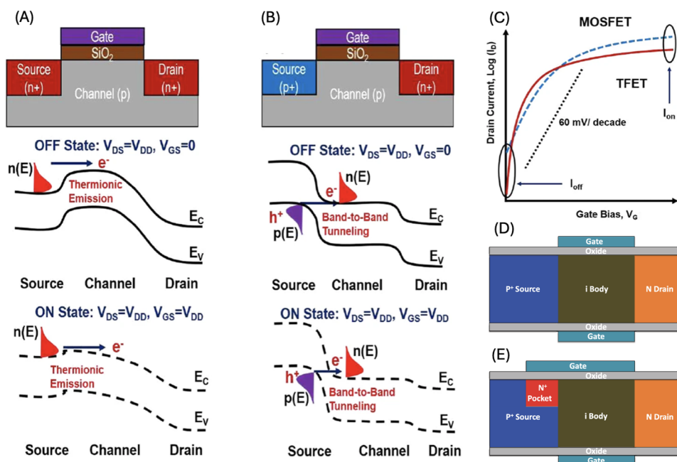
FIG. 1. Energy band diagram of (a) MOSFET, (b) TFET for on-state and off-state conditions, and (c) comparative transfer characteristics of well-designed MOSFET and TFET. Reproduced with permission from Kanungo et al. , npj 2D Mater. Appl. 6(1), 83 (2022). Copyright 2022 Nature Publishing Group. Schematic of simulated devices: (d) lateral InAs TFET and (e) vertical InAs TFET with a heavily doped n+ pocket (halo) in the gate-source overlap region. Reproduced with permission from Ganapathi et al. , Appl. Phys. Lett. 97, 033504 (2010). Copyright 2010 AIP Publishing LLC. 38
