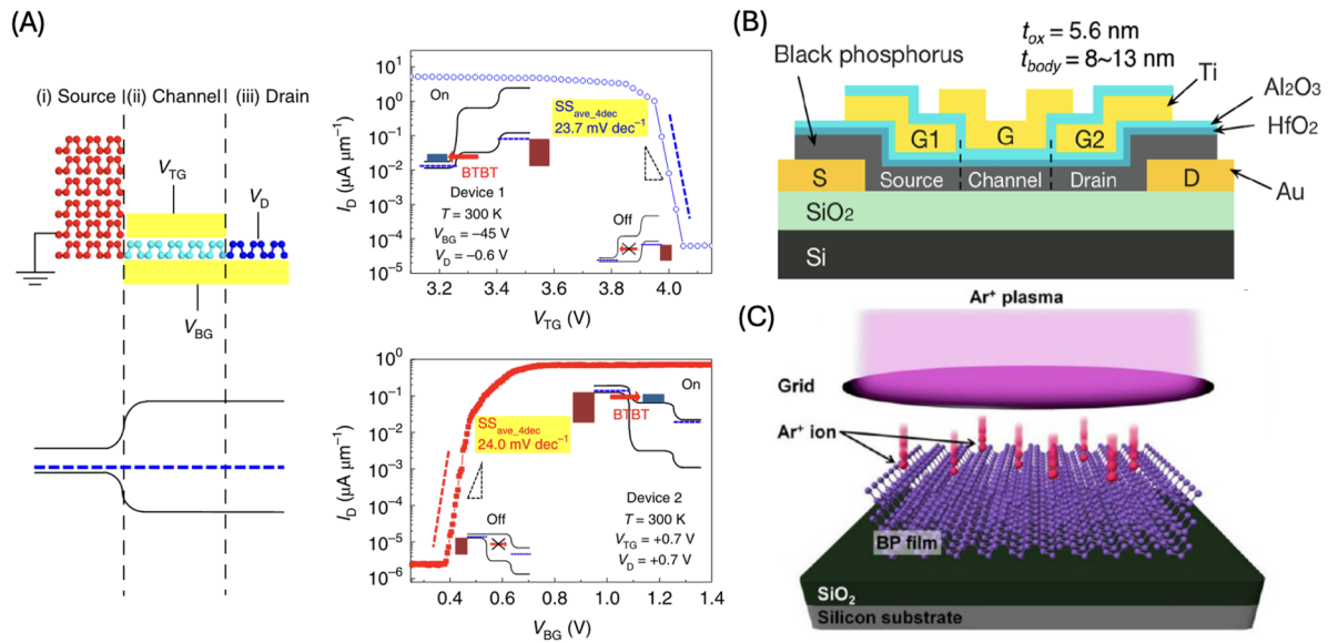
FIG. 4. (a) BP natural heterojunction (NHJ)-TFET schematic structure and BP band diagram in the (i) source, (ii) channel, and (iii) drain. Reproduced with permission from Kim et al. , Nat. Nanotechnol. 15 , 203–206 (2020). Copyright 2020 Nature Publishing Group. (b) Schematic of the BP reconfigurable electrostatically doped (RED) TFET. Reproduced with permission from Wu et al. , ACS Nano 13 , 377–385 (2019). Copyright 2019 American Chemical Society. (c) Schematic representation of the Ar + plasma treatment process to BP for defect-tailoring. Reproduced with permission from Kang et al. , ACS Photonics 4 , 1822–1830 (2017). Copyright 2017 American Chemical Society.
