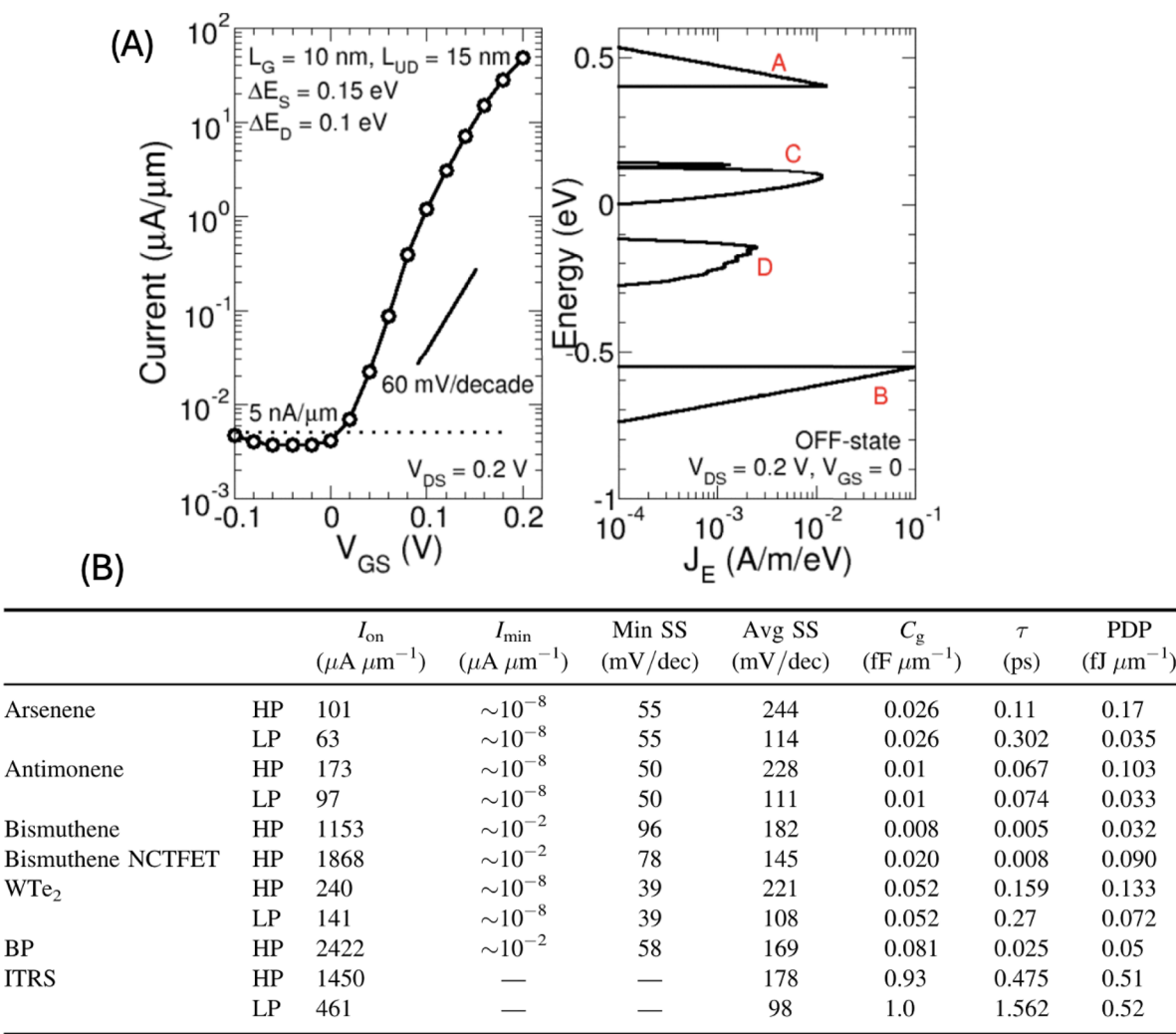
FIG. 6. (a) Left: Transfer characteristic of the n-type 2QL Bi 2 Se 3 TFET at V DS = 0.2V and room temperature, showing an effective SS of 50 mV/decade over 4 orders of magnitude. Right: Current spectrum in the off-state, demonstrating effective management of all four leakage components. Reproduced with permission from Zhang et al. , IEEE Electron Device Lett. 35 , 129–131 (2014). Copyright 2014 IEEE. (b) Benchmark comparison of ballistic device performances of ML group V-ene TFETs and ML bismuthene NCTFETs for high-performance (HP) and low-power (LP) applications, matched against the ITRS 2013 requirements. Also includes performance data for the ML WTe 2 TFET and ML BP TFET. Reproduced with permission from Li et al. , Semicond. Sci. Technol. 34 , 085006 (2019). Copyright 2019 IOP Publishing.
