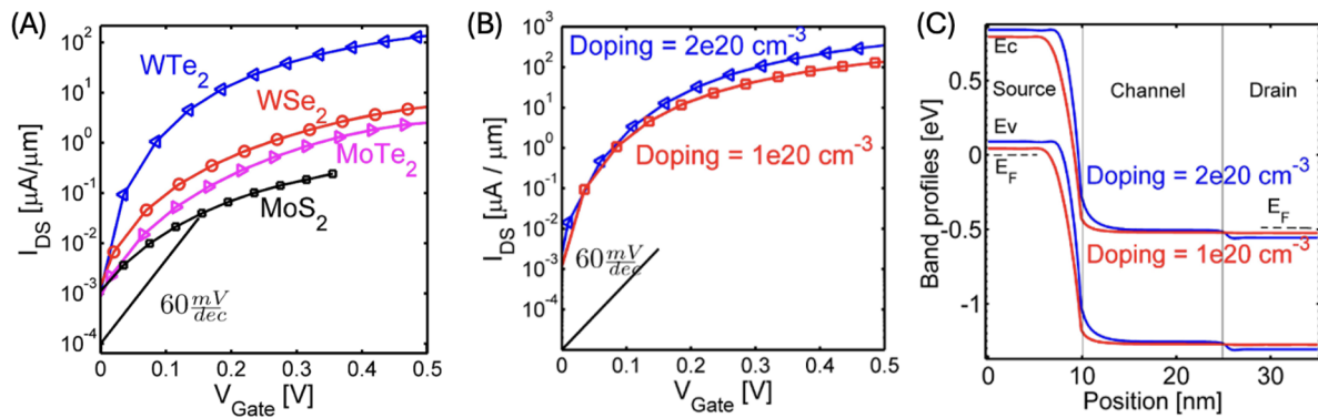
FIG. 3. High performance of TMD materials. (a) Transfer characteristics of TMD TFETs with I_{OFF} = 1 \text{ nA}/\mu\text{m} . (b) Transfer characteristics and (c) band diagrams of WTe 2 with doping levels of 1 \times 10^{20} and 2 \times 10^{20} \text{ cm}^{-3} . Reproduced with permission from Ilatikhameneh et al. , IEEE J. Explor. Solid-State Comput. Devices Circuits 1, 12–18 (2015). Copyright 2015 IEEE.
