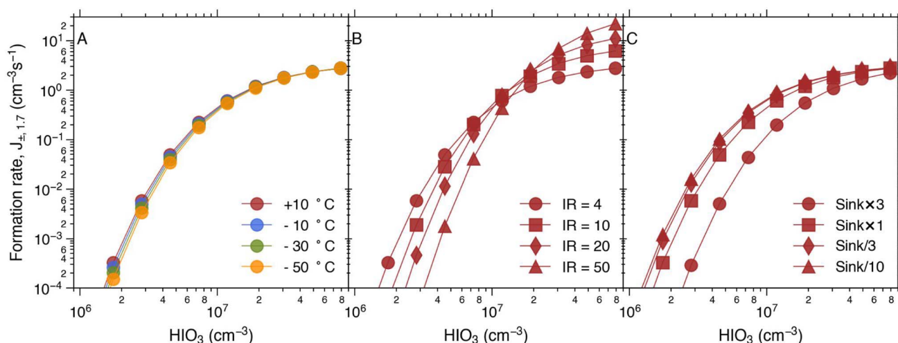
Fig. 3 The temperature (A), ionisation rate (B), and sink (C) dependence of J_{\pm} simulated by the PANDA520 model. If not stated otherwise the temperature is +10^\circ\text{C} , the ionisation rate is 4.1 \text{ ion pairs cm}^{-3} and the sink is 0.002 \text{ s}^{-1} . This shows that from these three parameters, the charged cluster formation rate is most sensitive to the ionisation rate. At \text{HIO}_3 concentrations below 1.5 \times 10^7 \text{ cm}^{-3} the impact of recombination loss is higher than the ion growth due to \text{HIO}_3 condensation and the formation rate decreases with increasing ionisation rate.
