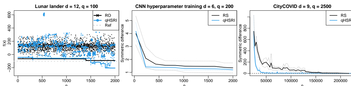
Figure 5: Left: optimality gap for the Lunar lander problem (one single run) with the evaluated values and estimated minimum found. Center: results of the tuning of the hyperparameters of a convolutional neural network over 5 macro-runs. Right: results on CityCOVID data set over 5 macro-runs. Thin dotted lines are 5% and 95% quantiles.
