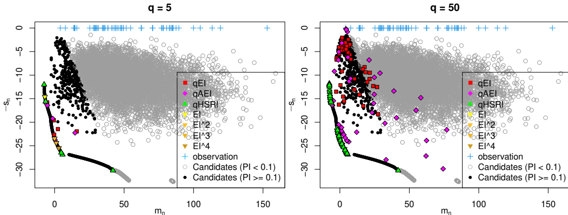
Figure 2: Comparison of qHSRI with qEI and qAEI acquisition functions on the noiseless repeated Branin function ( d = 6, n = 60 ). The first four GEI optimal solutions are depicted as well.
