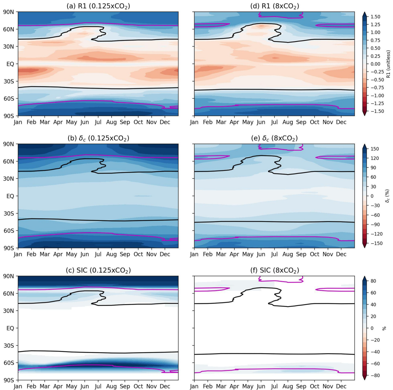
Figure 2. The spatio-temporal evolutions of panel (a) R_1 , (b) \delta_c , and (c) SIC in 0.125xCO 2 run. (d), (e), (f) show the same, but for the 8xCO 2 run. The magenta line indicates the boundary between the RAE and RCAE regimes, while the black line denotes the boundary separating the RCAE and RCE regimes.
