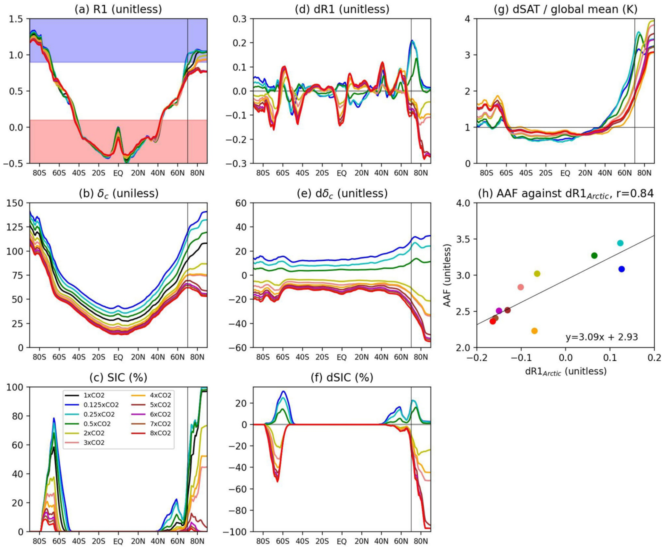
Figure 1. The latitudinal distributions for annual-mean zonal-mean (a) R_1 , (b) \delta_c , (c) SIC, (d) dR_1 , (e) d\delta_c , (f) dSIC , (g) dSAT divided by global means, and (h) AAF against dR_1 . The purple, white, and red shadings in panel (a) depict the RAE, RCAE, and RCE regimes, respectively. The units are denoted in the title of each panel.
