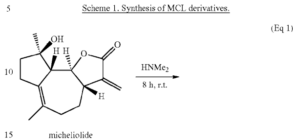
Scheme 1. Synthesis of MCL derivatives.
