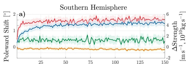
Figure 3. Time series of southern hemispheric response in model years to quadrupling atmospheric \text{CO}_2 for (a) the Hadley cell (HC) edge (red) and strength (orange) and the subtropical jet (STJ) location (green) and strength (blue). For each plot, shading represents the 95% confidence interval of model spread. Taken from Menzel et al. (2019).
