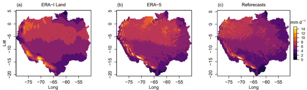
Figure 8. Mean daily precipitation totals throughout the Amazon basin. For (a) ERA-Interim Land, (b) ERA-5, and (c) the European Centre for Medium-Range Weather Forecasts (ECMWF) 20-year reforecasts. For the period 1997–2015.
