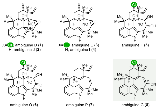
Figure 1. Selected members of the ambiguine natural products.
