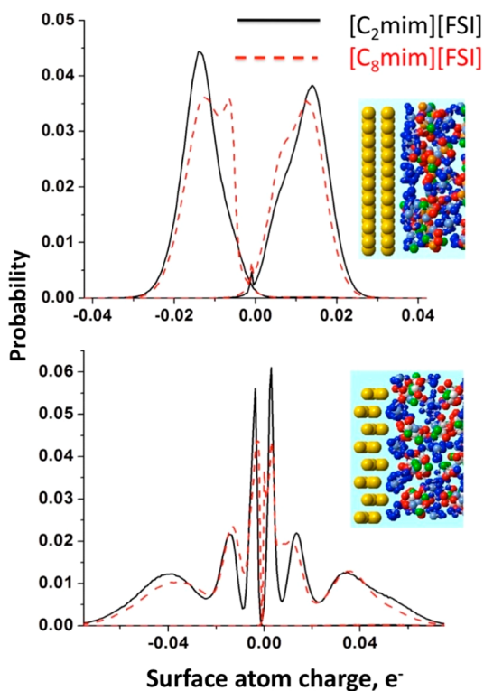
Figure 33. Distribution of instantaneous charges induced on electrode surface atoms as obtained from simulations using the constant applied potential for two ILs on atomically flat basal plane graphite (top) and atomically corrugated prismatic graphite (bottom). Reprinted with permission from ref 394. Copyright 2015 Elsevier.
