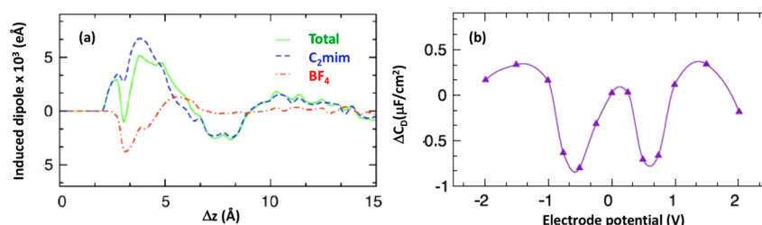
Figure 36. (a) The average induced dipole normal to the electrode surface in simulation [C 2 mim][BF 4 ] using a polarizable force field on atomically flat basal plane graphite using constant potential method. (b) Difference of differential capacitances obtained from simulations using polarizable nonpolarizable force fields for [C 2 mim][BF 4 ] in simulations with constant potential method. Adapted with permission from ref 430. Copyright 2016 American Institute of Physics.
