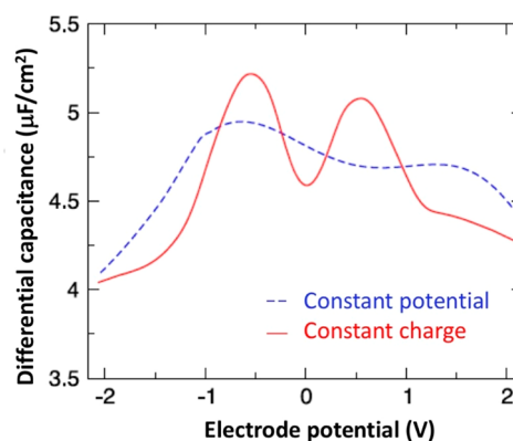
Figure 34. Differential capacitance as a function of electrode potential as obtained from MD simulations of [\text{C}_2\text{mim}][\text{BF}_4] on atomically flat basal plane graphite using constant charge and constant potential methods. Adapted with permission from ref 430. Copyright 2016 American Institute of Physics.
