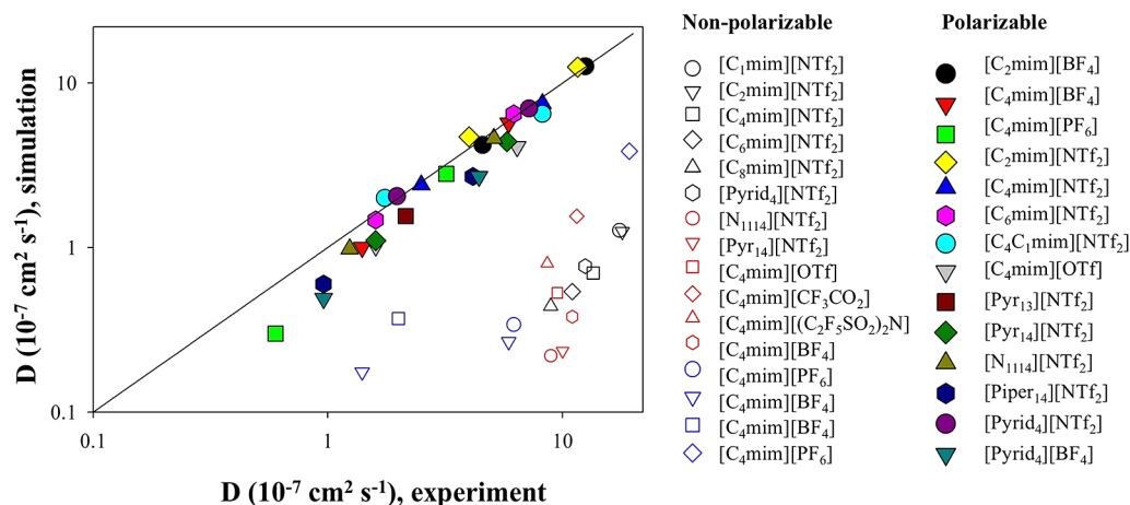
Figure 2. Correlation between averaged (for cation and anion) self-diffusion coefficients obtained from fully atomistic MD simulations and experimental data for several ionic liquids. Data for nonpolarizable force field are shown as open symbols and were compiled from several works where generic force fields were used without extended adjustments or modifications. For comparison, filled symbols show predictions of the generic polarizable force field. Data are compiled from refs 30, 47, and 44 and references therein.
