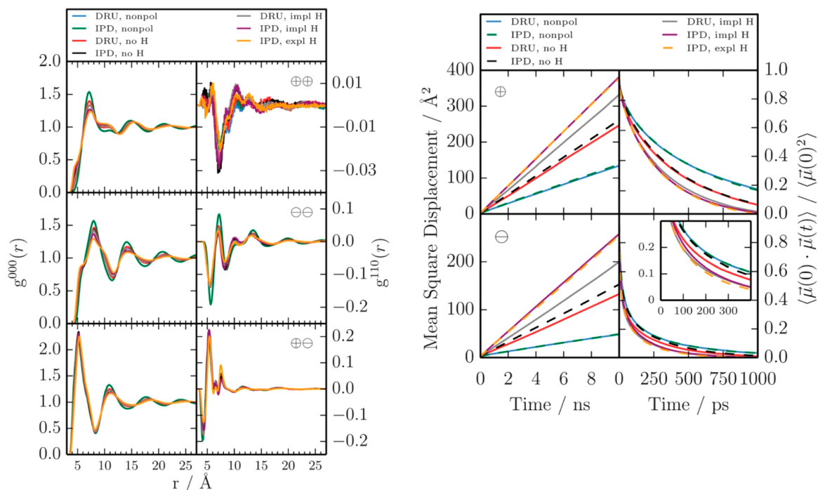
Figure 8. Structure and dynamics of [C 2 mim][OTf] from nonpolarizable and polarizable simulations using CHARMM (DRU) and AMBER (IPD). Reproduced with permission from ref 135. Copyright 2015 RCS Publishing.
