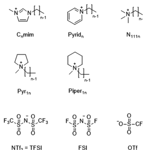
Figure 1. Typical ionic liquid cations and anions and their abbreviations used in this review. In the IL research community, \text{NTf}_2 is the common reference for this anion, while in the electrochemical community working with battery electrolytes, TFSI is the more common notation. Taking this into account, throughout the paper we will use both notations to be consistent with the most common usage in the discussed corresponding application.
