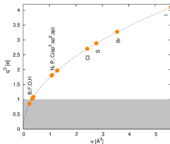
Figure 7. Drude charge of several polarizable atoms using a harmonic force constant k^D of 1000 kcal mol -1 Å -2 . Polarizabilities are taken from ref 145.
