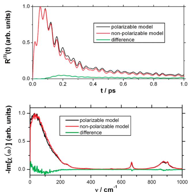
Figure 32. Anisotropic response function R^{(3)}(t) and OKE response function \chi(\omega) of polarizable and nonpolarizable [\text{C}_2\text{mim}][\text{NO}_3] simulations. 382 Reproduced from ref 382. Copyright 2010 American Chemical Society.
