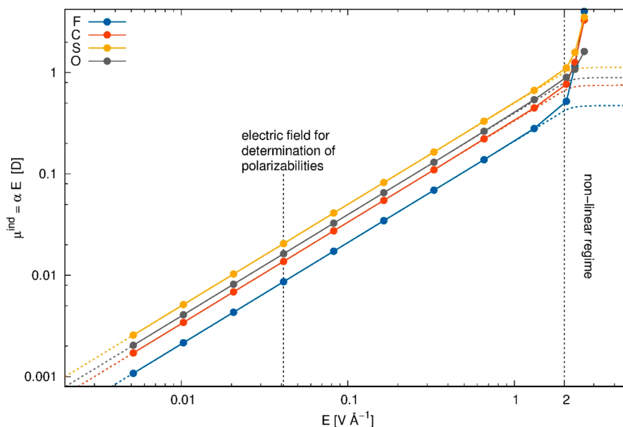
Figure 10. Atomic polarizabilities of OTf atoms as a function of the applied field. The values were determined via the AIM approach described in the next chapter. Additional details can be found in refs 195, 196.
