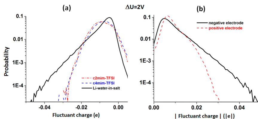
Figure 35. (a) The distribution of fluctuant charges for the graphite electrode top layer in contact to the electrolyte at a potential difference between electrodes of \Delta U = 2 V for the water-in-salt (WiSE) ( 21m LiNTf 2 + 7m LiOTf) electrolyte from MD simulations using a constant electrode potential methodology. 434 Solid black line compared electrode charges in contact with WiSE electrolyte and IL at similar surface voltage \varphi . A comparison of the fluctuant charge distribution for WiSE electrolyte studied here at the positive and negative electrode of a system at \Delta U = 2 V as a function of the positive part of the charge. 434 Reproduced from ref 434. Copyright 2017 American Chemical Society.
