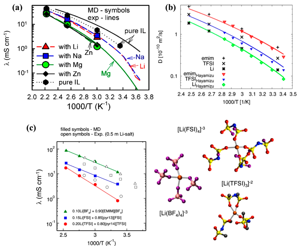
Figure 24. (a) Conductivity from the MD simulations (symbols) and experimental data (lines) of [Pyr 14 ][TFSI] doped with LiTFSI, NaTFSI, Mg(TFSI) 2 , and Zn(TFSI) 2 salts at metal:Pyr 14 = 1:4 ratio. 367 Reprinted from ref 367. Copyright 2018 American Chemical Society. (b) Diffusion coefficients for [C 2 mim][TFSI] + LiTFSI with C 2 mim:Li = 10.6 ratio from MD simulations 368 shown as black symbols, lines represent the Vogel–Tamman–Fulcher fit to experimental data, 368 the colored symbols show the diffusion coefficients determined by Hayamizu et al. 369 for m = 0.32 mol kg -1 . Reprinted from ref 368. Copyright 2014 American Chemical Society. (c) Ionic conductivity of [C 2 mim][BF 4 ] and [Pyr 14 ][TFSI] ILs doped with Li salts and snapshots of representative solvates from MD simulations using APPLE&P force field. 370 Reprinted from ref 370. Copyright 2014 American Chemical Society.
