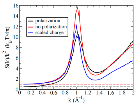
Figure 29. Reciprocal-space Coulomb interaction in [\text{C}_2\text{mim}][\text{BF}_4] computed with (black curve) and without (red curve) polarization and with scaled charges (blue curve). The dashed lines correspond to the long-range limit ( k = 0 ). Reproduced from ref 79. Copyright 2018 American Chemical Society.
