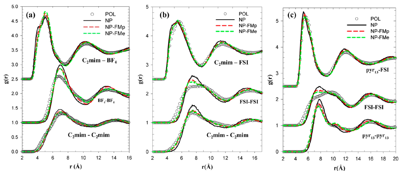
Figure 27. Ion center-of-mass radial distribution functions g(r) obtained from simulations using different force fields for [\text{C}_2\text{mim}][\text{BF}_4] , [\text{C}_2\text{mim}][\text{FSI}] , and [\text{Pyr}_{13}][\text{FSI}] ILs at atmospheric pressure and 393 K. 52 Reproduced from ref 52. Copyright 2010 American Chemical Society.
