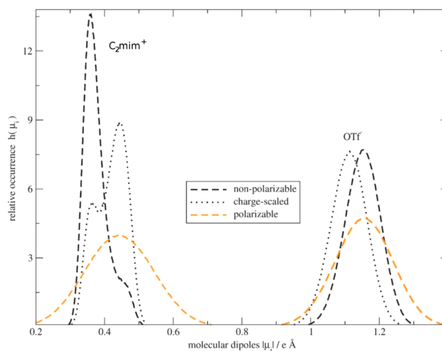
Figure 26. Histogram of molecular dipole moments of \text{C}_2\text{mim} and OTf for a nonpolarizable, charge-scaled, and polarizable simulation. Except for the charges and polarizabilities all other force field parameters were kept fixed. Reproduced with permission from ref 45. Copyright 2012 RSC Publishing.
