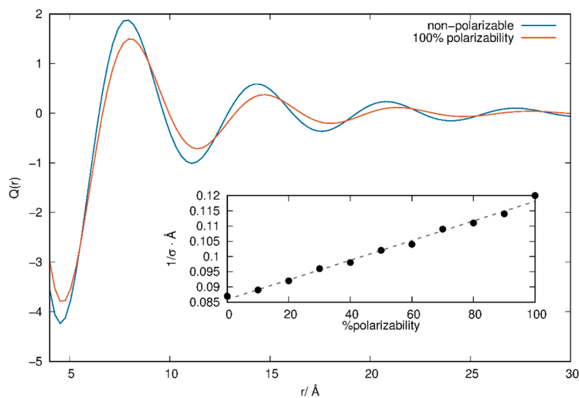
Figure 28. Charge ordering function Q(r) (see eq 3.3.1) of [\text{C}_2\text{mim}][\text{OTf}] using a polarizable and nonpolarizable force field. 135
