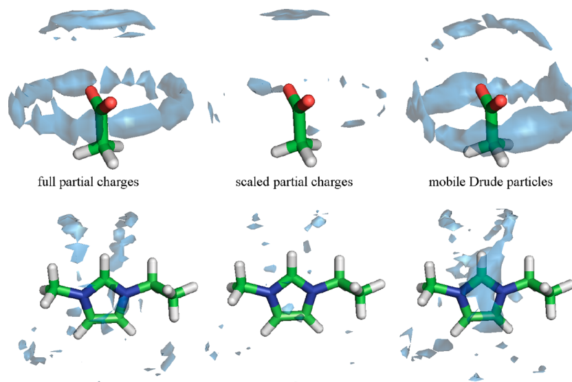
Figure 25. Hydrogen bonding in various MD simulations of aqueous [\text{C}_2\text{mim}][\text{acetate}] mixtures using full and scaled partial charges as well as a polarizable force field. The blue areas depict favorable positions of the water hydrogens.
