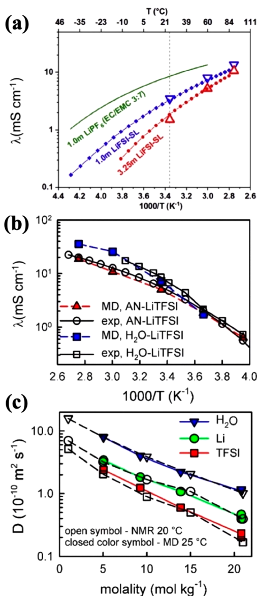
Figure 23. (a) Temperature dependence of ionic conductivity in SL-based electrolyte doped with 1 m and 3.25 m of LiFSI salt obtained from experiments (shown as lines) and MD simulation predictions using the polarizable APPLE&P force field (large triangle symbols) from Alvarado et al. 257 Reprinted with permission from ref 257. Copyright 2018 Elsevier. (b) Temperature dependence of conductivity from MD simulations and experiments for AN:LiTFSI electrolyte with AN:Li = 3 from Seo et al. 360 and H 2 O:LiTFSI electrolyte with H 2 O:Li = 2.67 from Borodin et al. 258 (c) Self-diffusion coefficients of Li + , TFSI, and H 2 O as a function of salt concentration in H 2 O:LiTFSI electrolytes from MD simulations and PFG-NMR experiments. 258 Reprinted from ref 258. Copyright 2017 American Chemical Society.
