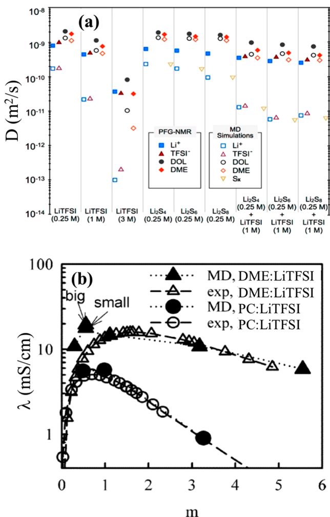
Figure 21. (a) Self-diffusion coefficients of solvents and ions in the 1,3-dioxalane (DOL): dimethoxy ethane (DME) electrolytes with 0.25 M, 1 M, or 3 M LiTFSI, 0.25 M Li 2 S x ( x = 4, 6, 8), and 0.25 M Li 2 S x ( x = 4, 6, 8) + 1 M LiTFSI salts computed from MD simulations and PFG-NMR. 43 Reproduced with permission from ref 43. Copyright 2017 American Chemical Society. (b) Conductivity of DME:LiTFSI and PC:LiTFSI electrolytes as a function of salt concentration expressed in mol per kg solvent ( m ) as obtained from experiments and from MD simulations using a many-body polarizable force field. 246 Reproduced with permission from ref 246. Copyright 2006 American Chemical Society.
