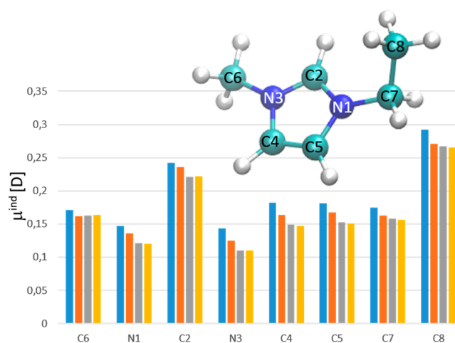
Figure 6. Induced atomic dipoles of several atoms in 1-ethyl-3-methylimidazolium as a function of the Drude charge q^D . Blue, orange, gray, and yellow represent -0.5e , -1.0e , -2.0e , and -4.0e , respectively. 122
