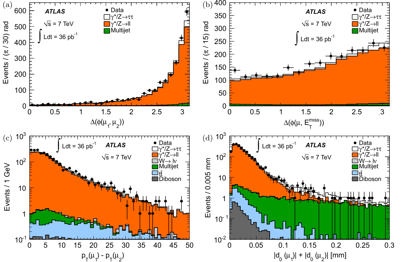
FIG. 9 (color online). Distributions of some of the input variables to the BDT used to optimize the selection of the \tau_\mu\tau_\mu final state. The data are compared to signal ( \gamma^*/Z \rightarrow \tau\tau ) and \gamma^*/Z \rightarrow \mu\mu Monte Carlo samples. The multijet background is estimated from data (see Sec. V). The observed differences are consistent with the estimated systematic uncertainties on the \gamma^*/Z background normalization.
