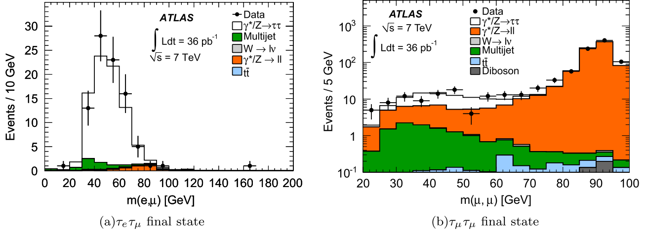
FIG. 7 (color online). The distributions of the visible mass for the (a) \tau_e \tau_\mu and (b) \tau_\mu \tau_\mu final states, after all selections except the selection on the visible mass.
