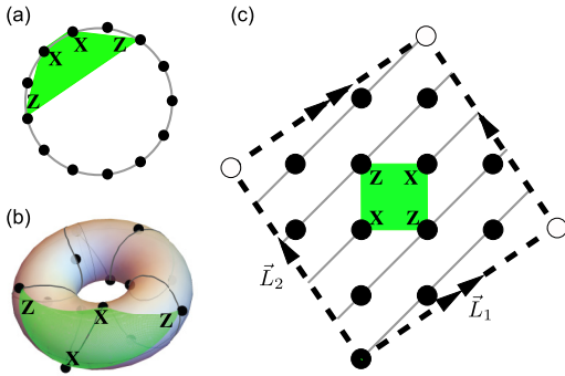
FIG. 1. Map from the S(13, 2, 1) code (a) to a GTC with \vec{L}_1 = (3, 2) , \vec{L}_2 = (-2, 3) [(b),(c)]. The qubits are represented by black dots and labeled along the solid-grey string. The stabilizer generators are represented by green plaquettes (only one generator is plotted and others are obtained by shifting along the grey string). [(b),(c)] Obtained by wrapping the grey string around the torus. (c) The 2D layout of (b), with opposite sides of the parallelogram enclosed by \vec{L}_1, \vec{L}_2 identified.
