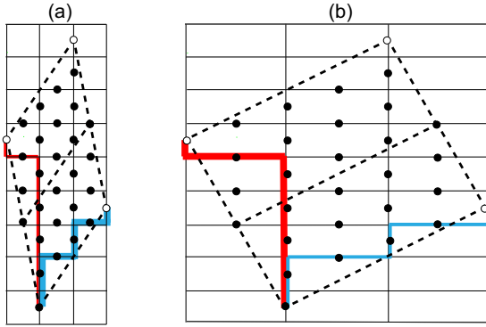
FIG. 3. Geometric representation of the logical operators of the [[13, 1, 5]] GTC with \vec{L}_1 = (-1, 5) = 2\hat{x} + 3\hat{z} , \vec{L}_2 = (-3, 2) = -\frac{1}{2}\hat{x} + \frac{5}{2}\hat{z} for (a) \omega = 1 and (b) \omega = 3 . The horizontal and vertical axes are aligned with the X and Z axes, respectively. The doubled graph is obtained by doubling along \vec{L}_2 : \vec{L}_{1,d} = \vec{L}_1 , \vec{L}_{2,d} = 2\vec{L}_2 = -\hat{x} + 5\hat{z} . The blue (red) cycle represents the logical operator associated with \vec{L}_{1,d} ( \vec{L}_{2,d} ). The shortest nontrivial cycles \vec{L}_m in the modified 1-norm determined by Eq. (3) are thickened. For (a) \omega = 1 , \vec{L}_m = \vec{L}_{1,d} and d' = \|\vec{L}_{1,d}\|_{xz,1} = 5 ; For (b) \omega = 3 , \vec{L}_m = \vec{L}_{2,d} and d' = \|\vec{L}_{2,d}\|_{xz,1} = 8 .
