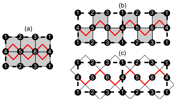
FIG. 2. The construction of doubled graph for a non-two-colorable GTC with \vec{L}_1 = (0, 2), \vec{L}_2 = (3, 0) . (a) The original non-two-colorable graph G that defines the GTC. There is a XZZX stabilizer on each of the shaded plaquettes. The red cycle depicts a logical operator Y_4Y_5Y_6 that cannot wrap back on itself after a single loop due to odd periodicity in the horizontal direction. (b) The doubled graph G_d obtained by taking two copies of G and gluing them horizontally. Now G_d becomes two colorable and the stabilizers are only put on the shaded plaquettes. Consequently, a single loop is sufficient for the logical operator to wrap back on itself. (c) The equivalent graph G'_d of G_d where qubits are placed on the edges and stabilizers are placed on the vertices. Now the logical operator corresponds to a well-defined cycle that is homologically nontrivial on the doubled torus.
