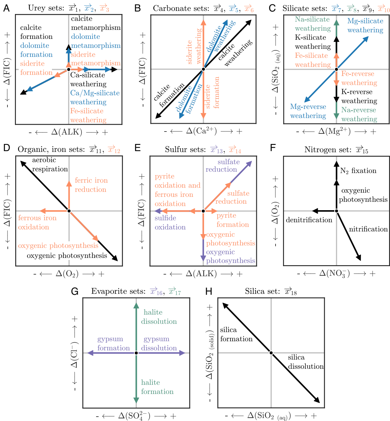
Fig. 3. Closed sets. These mutually canceling combinations of biogeochemical reactions are grouped into categories describing (A) Urey-style reactions, (B) carbonate weathering and formation, (C) silicate weathering and reverse weathering, (D–F) cycling of organic matter, iron, sulfur, pyrite, and nitrogen, (G and H) dissolution and formation of gypsum, halite, and silica. Each closed set can be combined at arbitrary magnitudes with the other closed sets without destabilizing major element cycles. Within each panel, the biogeochemical processes contributing to individual sets are presented in the same color. The plotted scaling for each set is to enhance visibility and does not reflect relative importance in the Earth system.
