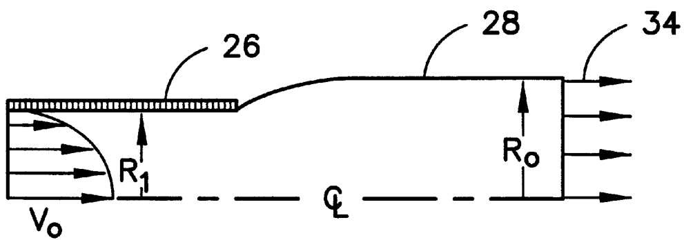
FIG. 3 (PRIOR ART)
