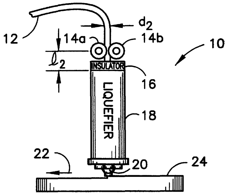
FIG. 1 (PRIOR ART)
