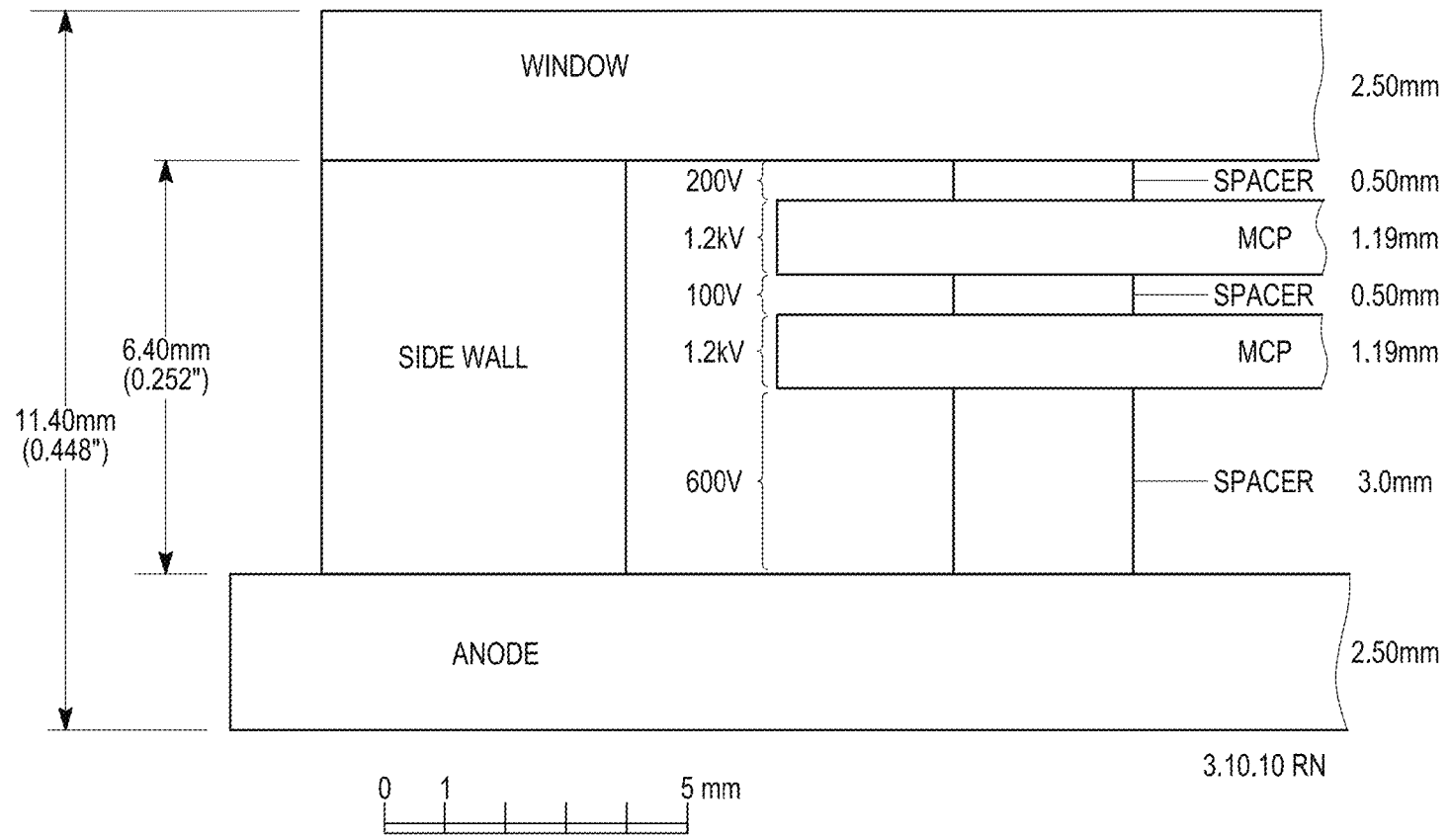
BASE LINE MCP-PMT STACKUP
