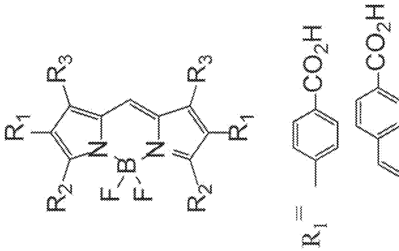
BODIPY derivatives
