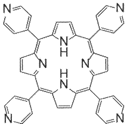
5,10,15,20-tetra(p-pyridyl)porphyrin
