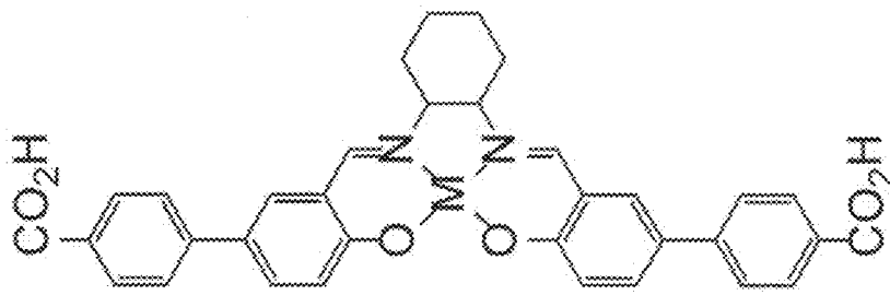
disalicylidene-1,2-cyclohexylidenediamine complex
