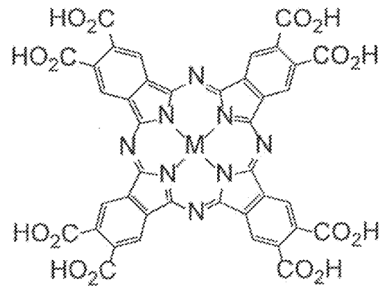
Phthalocyanine-octacarboxylic acid
