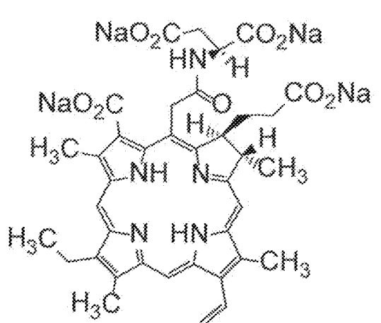
NPe6 (Talaporfin)
