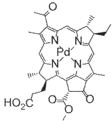
Padoporphin (Tookad)
