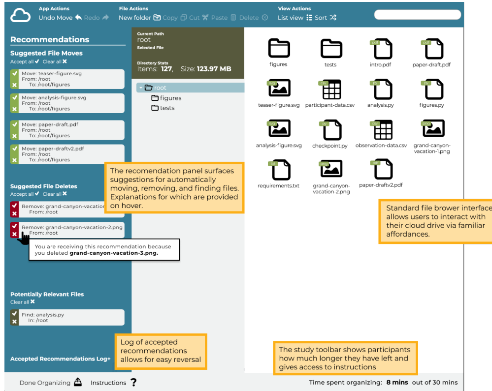
Figure 1.1: A screenshot of our semi-automated file-management tool, KondoCloud, discussed in Chapter 4.
