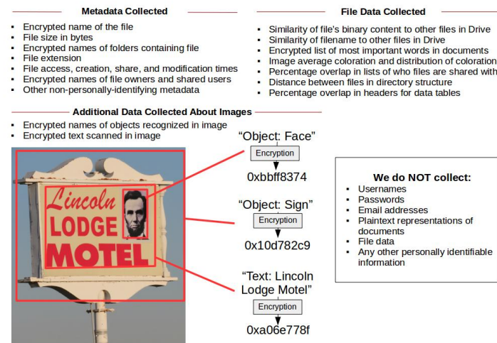
Figure A.1: Image displayed to participants before allowing our web application access to their cloud accounts
