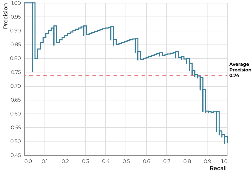
Figure 4.8: Precision-recall curve for the overall classifier.
