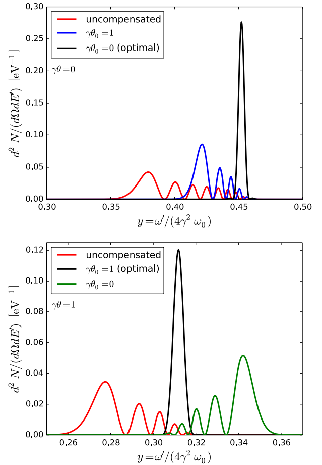
FIG. 4. Top: Radiation spectrum for the compensated nonlinear Compton backscattering ( \theta = 0 ). The optimally compensated spectrum shown in black for \theta_0 = \theta is much narrower than the uncompensated spectrum (red line) and partially compensated spectrum (blue line), where the optimization angle \theta_0 does not coincide with the scattering angle \theta . Bottom: Radiation spectra for the compensated nonlinear Compton scattering at an angle \theta = 1/\gamma and \phi = \pi/2 . The optimally compensated spectrum is shown in black for \theta_0 = \theta = 1/\gamma , uncompensated in red and the spectrum for which the optimization angle does not coincide with the scattering angle ( \theta_0 = 0 ) in green. Top and bottom panels are to be compared with Figs. 2(a) and 2(b) from Ref. [8], respectively. Our spectra assume both positive and negative frequencies exist in the spectra; Ref. [8] assumes positive frequency only and is therefore a factor of 2 higher. Both plots are for the head-on scattering of a linearly polarized 800 nm laser with pulse duration of 21 fs and a_0 = 1 on an electron beam with initial energy 51 GeV. A Gaussian laser envelope is used.
