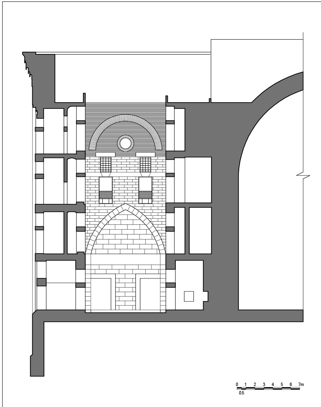
Fig. 10. Shāfiʿīyah Madrasah, Complex of Sultan Ḥasan, Cairo, section CC (H. Al-Harithy)
